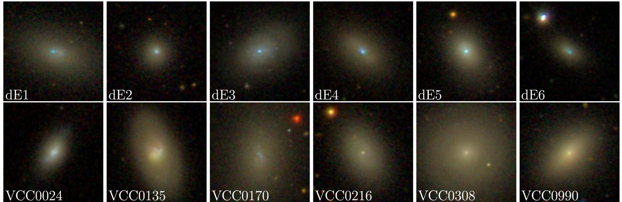
Figure 1. from Starbursting Nuclei in Old Dwarf Galaxies null 2020 APJL 898 L47 doi:10.3847/2041-8213/aba6ed http://dx.doi.org/10.3847/2041-8213/aba6ed © 2020. The American Astronomical Society. All rights reserved.
