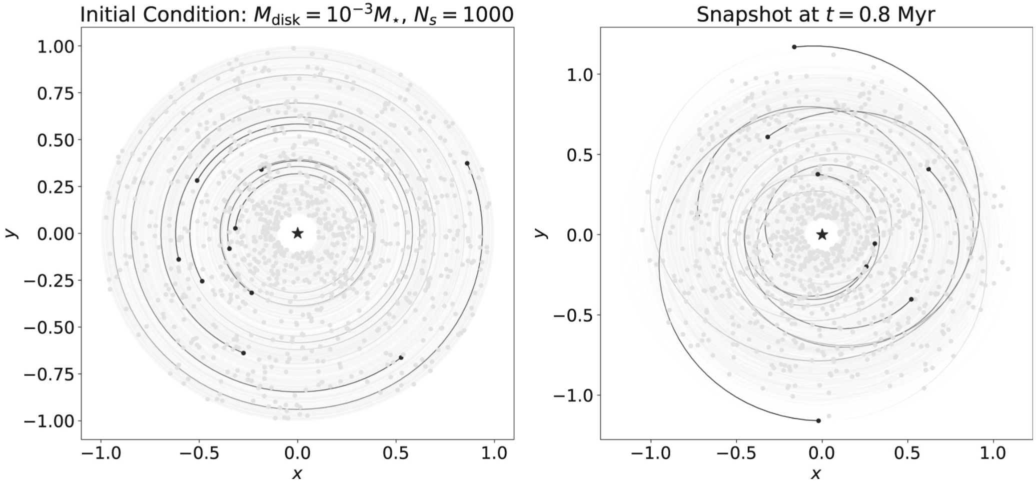
Figure 1. from Interactions among Noninteracting Particles in Planet Formation Simulations null 2020 APJL 898 L46 doi:10.3847/2041-8213/aba68d http://dx.doi.org/10.3847/2041-8213/aba68d © 2020. The American Astronomical Society. All rights reserved.
