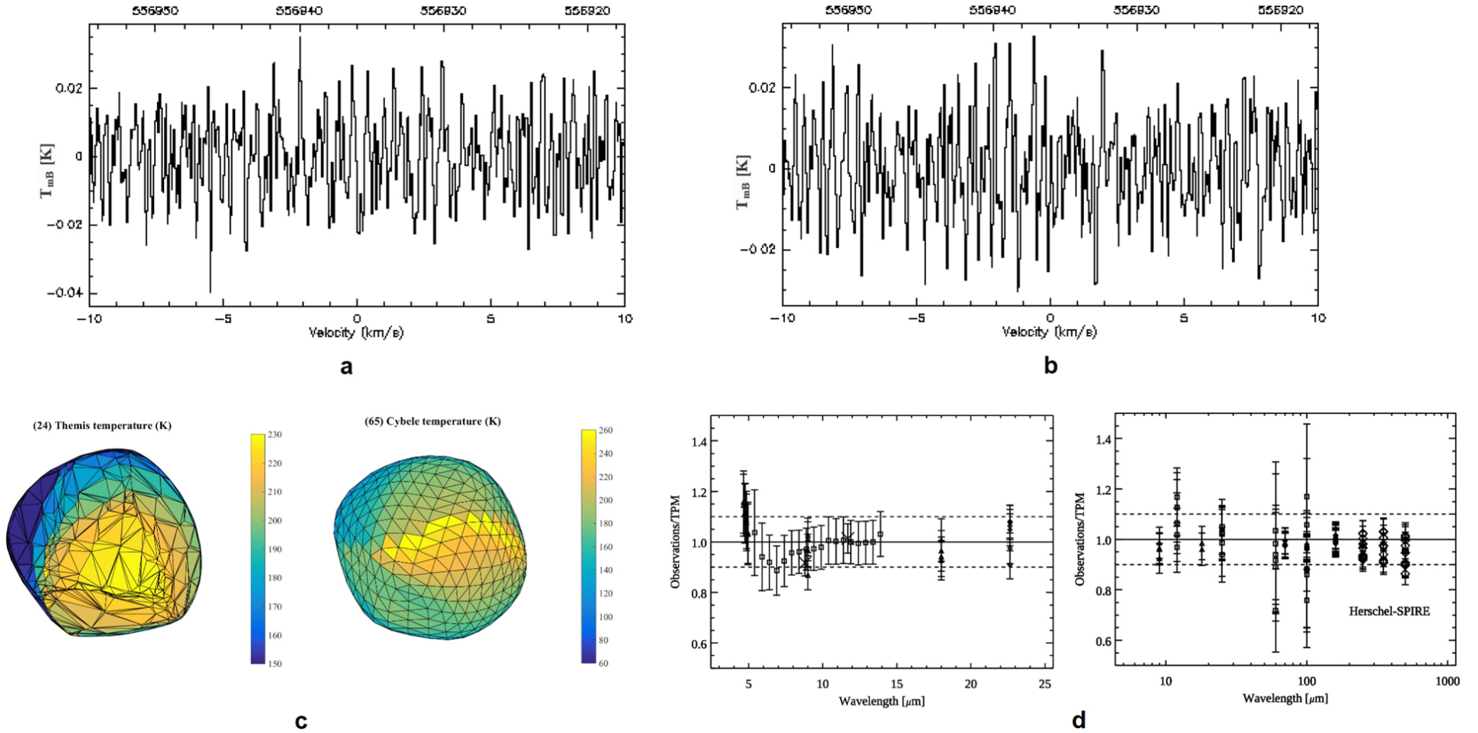
Figure 1. from Low Water Outgassing from (24) Themis and (65) Cybele: 3.1 m Near-IR Spectral Implications null 2020 APJL 898 L45 doi:10.3847/2041-8213/aba62b http://dx.doi.org/10.3847/2041-8213/aba62b © 2020. The American Astronomical Society. All rights reserved.
