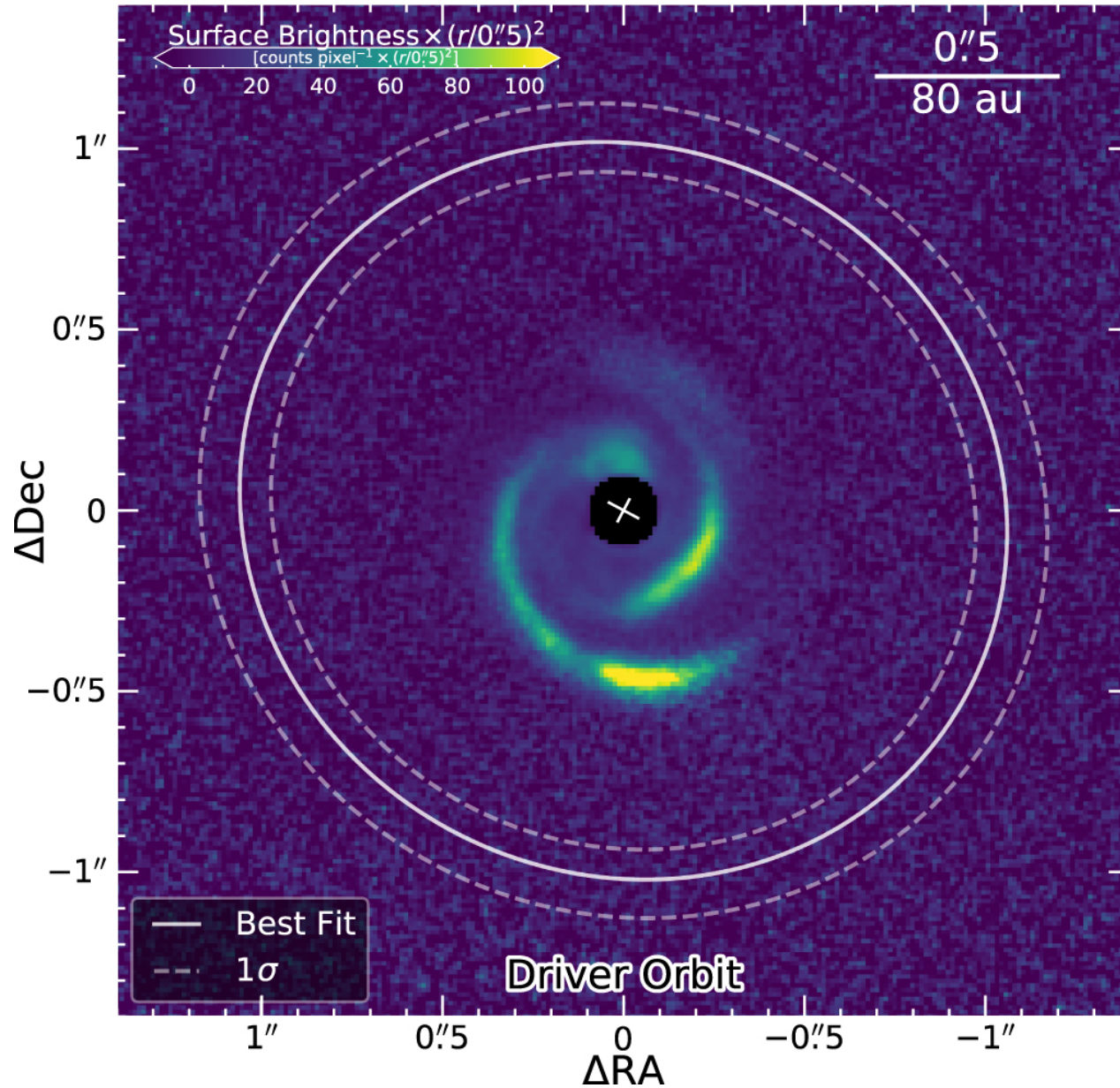
Figure 3. from Dynamical Evidence of a Spiral Arm–driving Planet in the MWC 758 Protoplanetary Disk null 2020 APJL 898 L38 doi:10.3847/2041-8213/aba43e http://dx.doi.org/10.3847/2041-8213/aba43e © 2020. The American Astronomical Society. All rights reserved.
