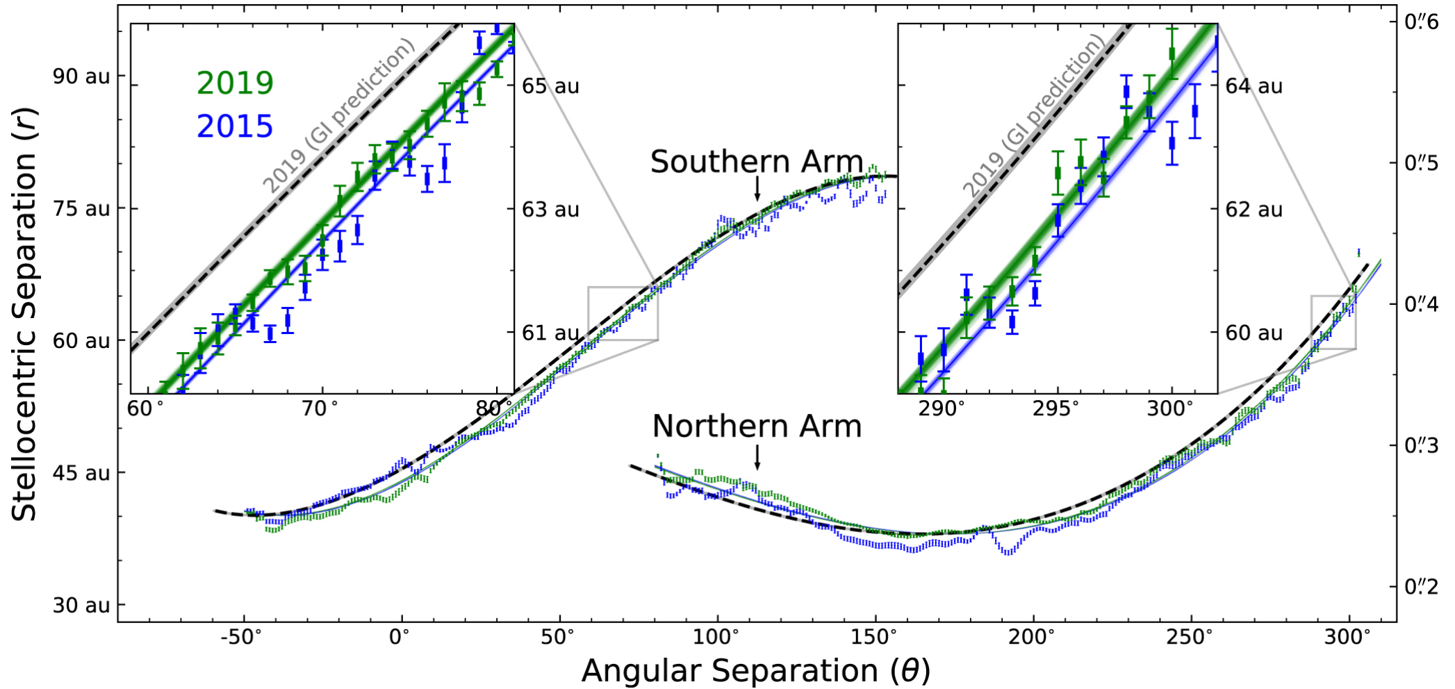
Figure 2. from Dynamical Evidence of a Spiral Arm–driving Planet in the MWC 758 Protoplanetary Disk null 2020 APJL 898 L38 doi:10.3847/2041-8213/aba43e http://dx.doi.org/10.3847/2041-8213/aba43e © 2020. The American Astronomical Society. All rights reserved.
