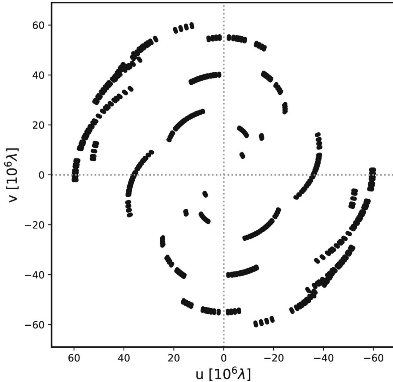
Figure 1. from Spin–Orbit Alignment of the Pictoris Planetary System null 2020 APJL 897 L8 doi:10.3847/2041-8213/ab9d27 http://dx.doi.org/10.3847/2041-8213/ab9d27 © 2020. The American Astronomical Society. All rights reserved.
