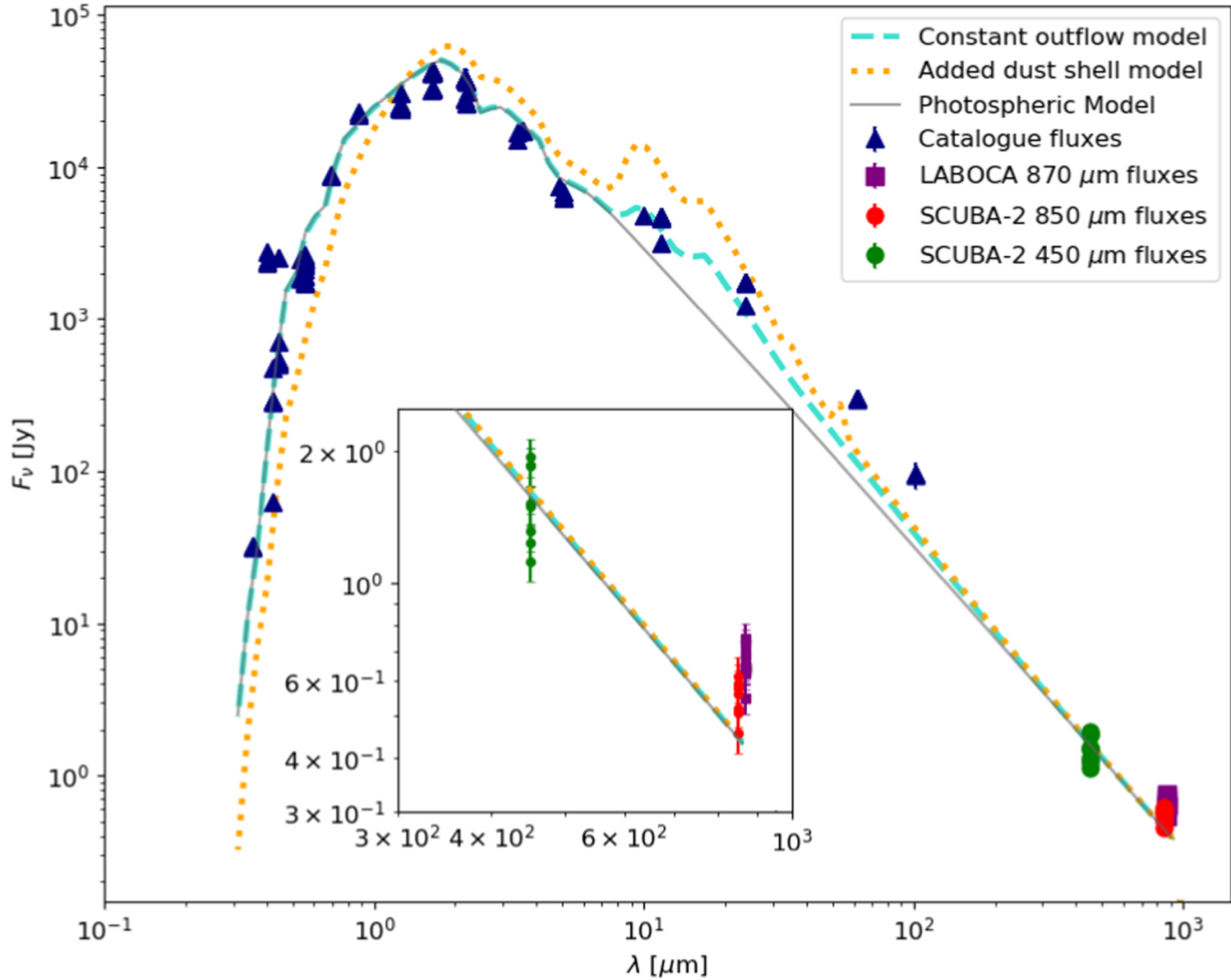
Figure 2. from Betelgeuse Fainter in the Submillimeter Too: An Analysis of JCMT and APEX Monitoring during the Recent Optical Minimum null 2020 APJL 897 L9 doi:10.3847/2041-8213/ab9ca6 http://dx.doi.org/10.3847/2041-8213/ab9ca6 © 2020. The American Astronomical Society. All rights reserved.
