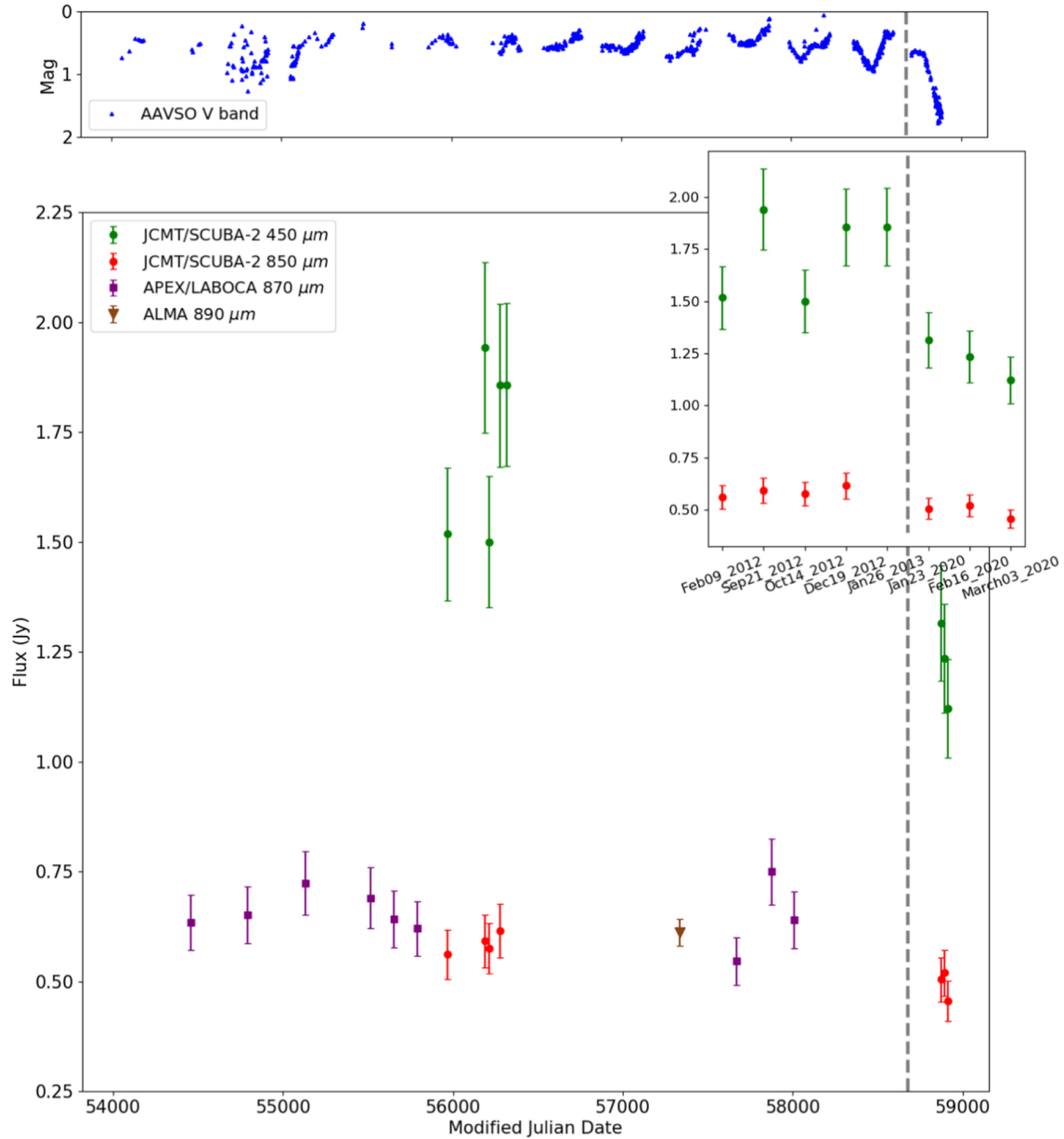
Figure 1. from Betelgeuse Fainter in the Submillimeter Too: An Analysis of JCMT and APEX Monitoring during the Recent Optical Minimum null 2020 APJL 897 L9 doi:10.3847/2041-8213/ab9ca6 http://dx.doi.org/10.3847/2041-8213/ab9ca6 © 2020. The American Astronomical Society. All rights reserved.
