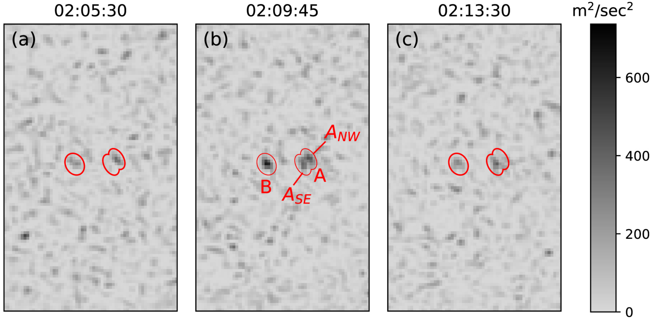
Figure 4. from Ultra-impulsive Solar Flare Seismology null 2020 APJL 895 L19 doi:10.3847/2041-8213/ab9173 http://dx.doi.org/10.3847/2041-8213/ab9173 © 2020. The American Astronomical Society. All rights reserved.
