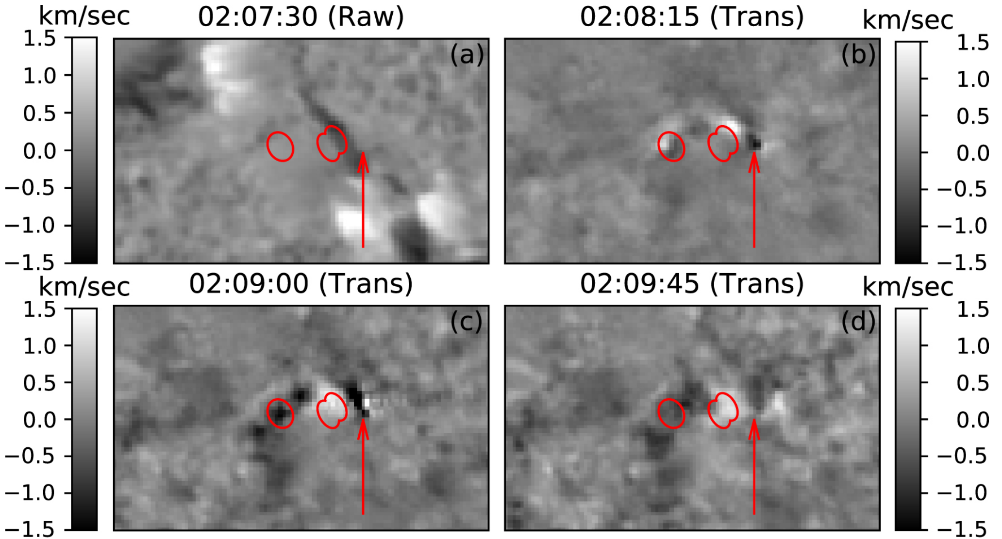
Figure 3. from Ultra-impulsive Solar Flare Seismology null 2020 APJL 895 L19 doi:10.3847/2041-8213/ab9173 http://dx.doi.org/10.3847/2041-8213/ab9173 © 2020. The American Astronomical Society. All rights reserved.
