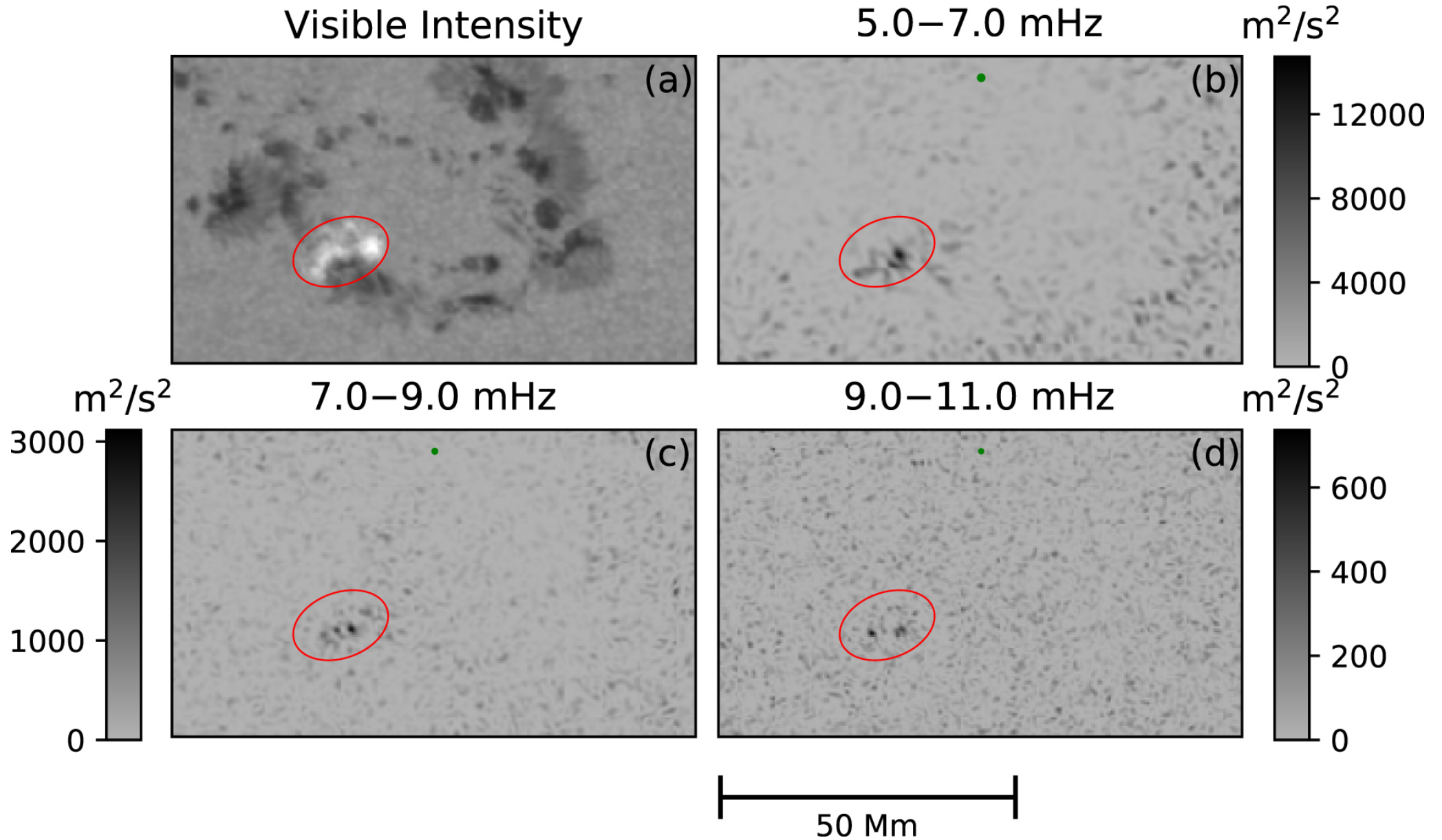
Figure 1. from Ultra-impulsive Solar Flare Seismology null 2020 APJL 895 L19 doi:10.3847/2041-8213/ab9173 http://dx.doi.org/10.3847/2041-8213/ab9173 © 2020. The American Astronomical Society. All rights reserved.
