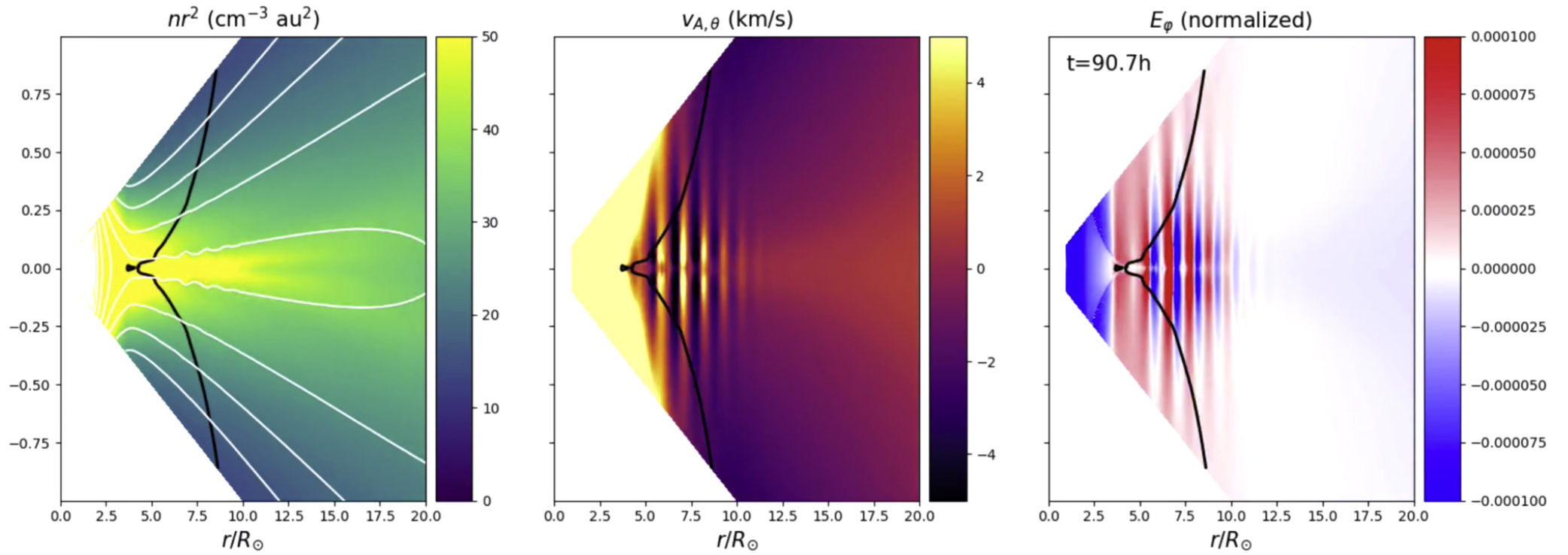
Figure A1. from Tearing Instability and Periodic Density Perturbations in the Slow Solar Wind null 2020 APJL 895 L20 doi:10.3847/2041-8213/ab911d http://dx.doi.org/10.3847/2041-8213/ab911d © 2020. The Author(s). Published by the American Astronomical Society.
