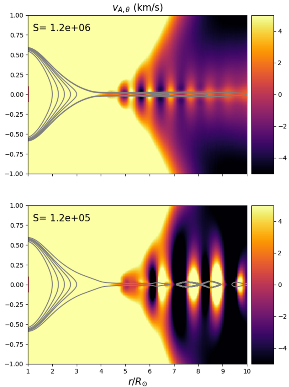
Figure 3. from Tearing Instability and Periodic Density Perturbations in the Slow Solar Wind null 2020 APJL 895 L20 doi:10.3847/2041-8213/ab911d http://dx.doi.org/10.3847/2041-8213/ab911d © 2020. The Author(s). Published by the American Astronomical Society.
