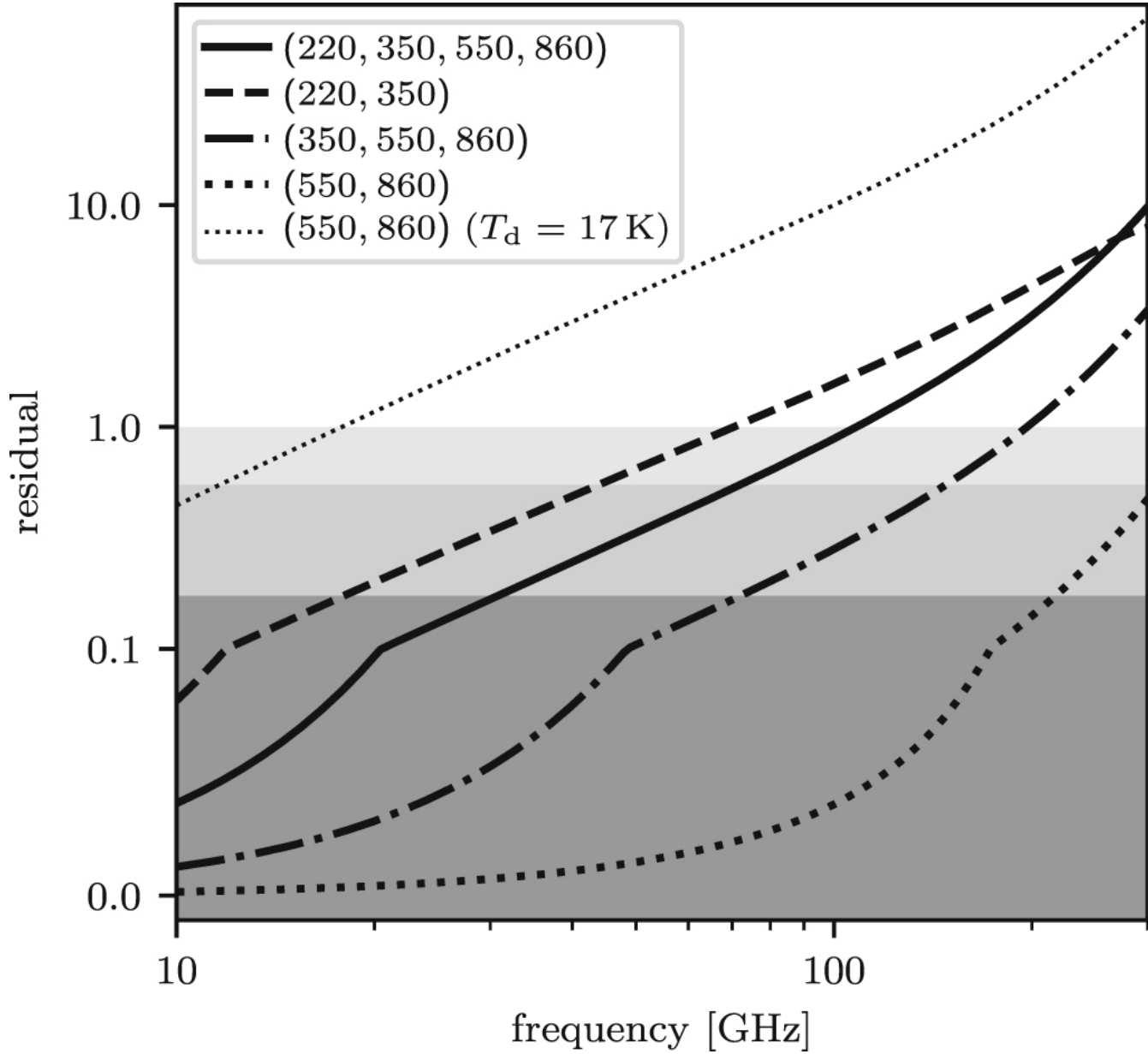
Figure 4. from CMB Shadows: The Effect of Interstellar Extinction on Cosmic Microwave Background Polarization and Temperature Anisotropy null 2020 APJL 895 L21 doi:10.3847/2041-8213/ab9018 http://dx.doi.org/10.3847/2041-8213/ab9018 © 2020. The American Astronomical Society. All rights reserved.
