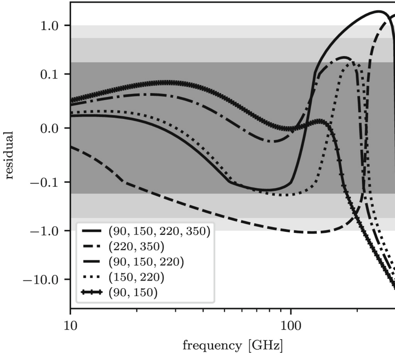
Figure 3. from CMB Shadows: The Effect of Interstellar Extinction on Cosmic Microwave Background Polarization and Temperature Anisotropy null 2020 APJL 895 L21 doi:10.3847/2041-8213/ab9018 http://dx.doi.org/10.3847/2041-8213/ab9018 © 2020. The American Astronomical Society. All rights reserved.
