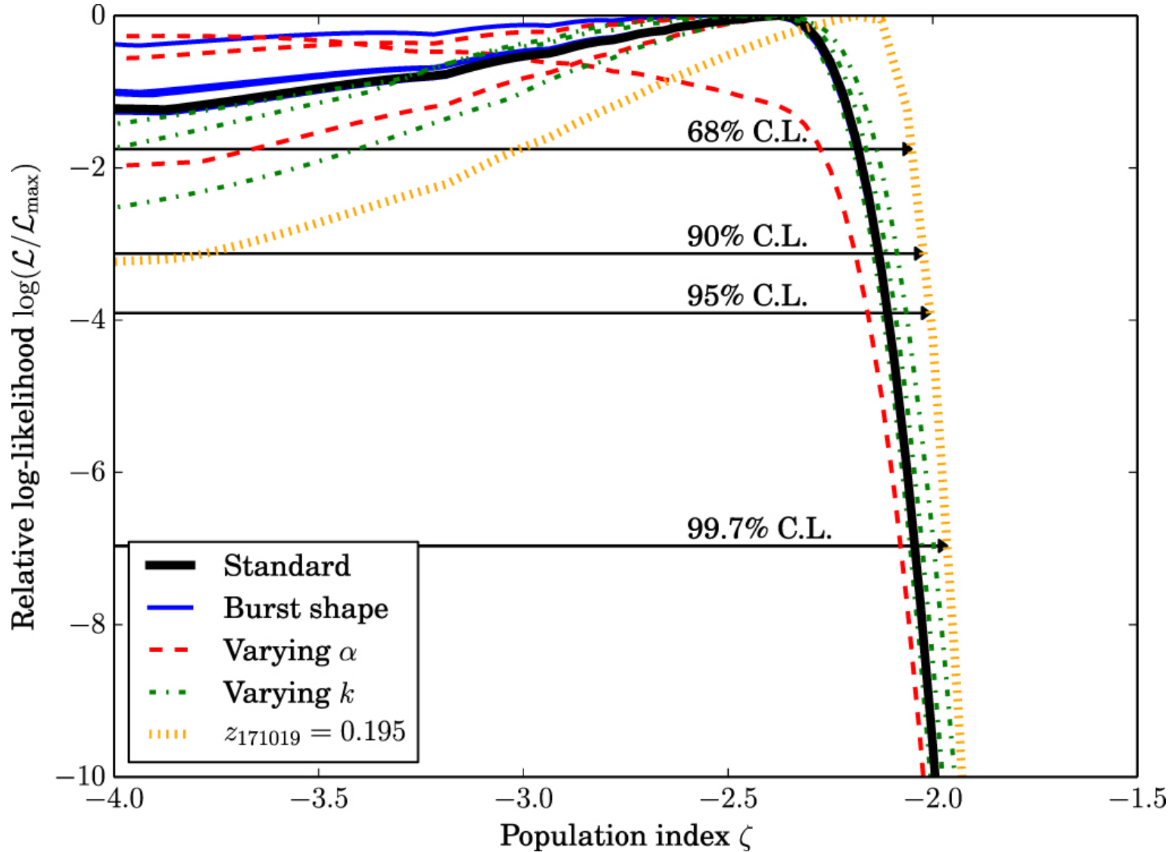
Figure 2. from Measurement of the Rate Distribution of the Population of Repeating Fast Radio Bursts: Implications for Progenitor Models null 2020 APJL 895 L22 doi:10.3847/2041-8213/ab8f99 http://dx.doi.org/10.3847/2041-8213/ab8f99 © 2020. The American Astronomical Society. All rights reserved.
