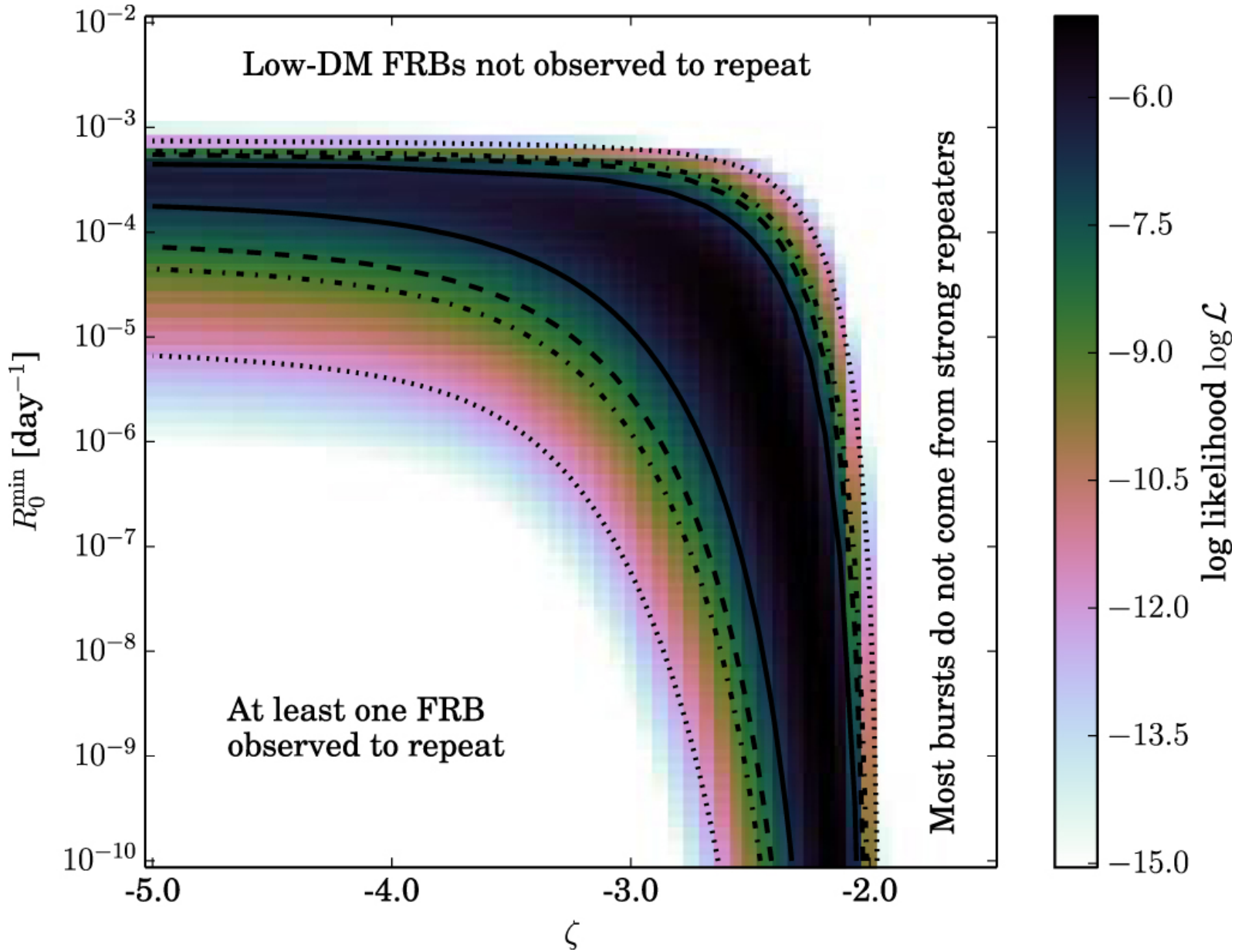
Figure 1. from Measurement of the Rate Distribution of the Population of Repeating Fast Radio Bursts: Implications for Progenitor Models null 2020 APJL 895 L22 doi:10.3847/2041-8213/ab8f99 http://dx.doi.org/10.3847/2041-8213/ab8f99 © 2020. The American Astronomical Society. All rights reserved.
