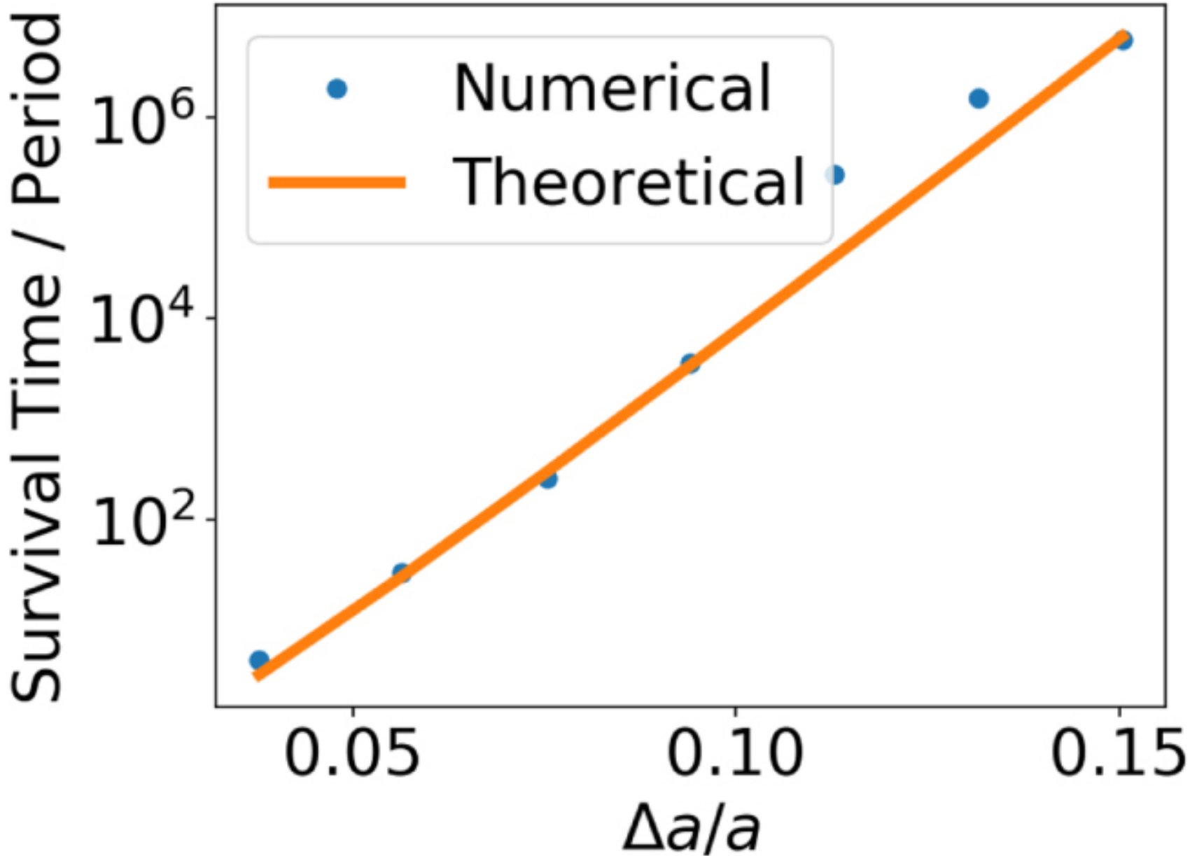
Figure 2. from Nekhoroshev Estimates for the Survival Time of Tightly Packed Planetary Systems null 2020 APJL 892 L11 doi:10.3847/2041-8213/ab75dc http://dx.doi.org/10.3847/2041-8213/ab75dc © 2020. The American Astronomical Society. All rights reserved.
