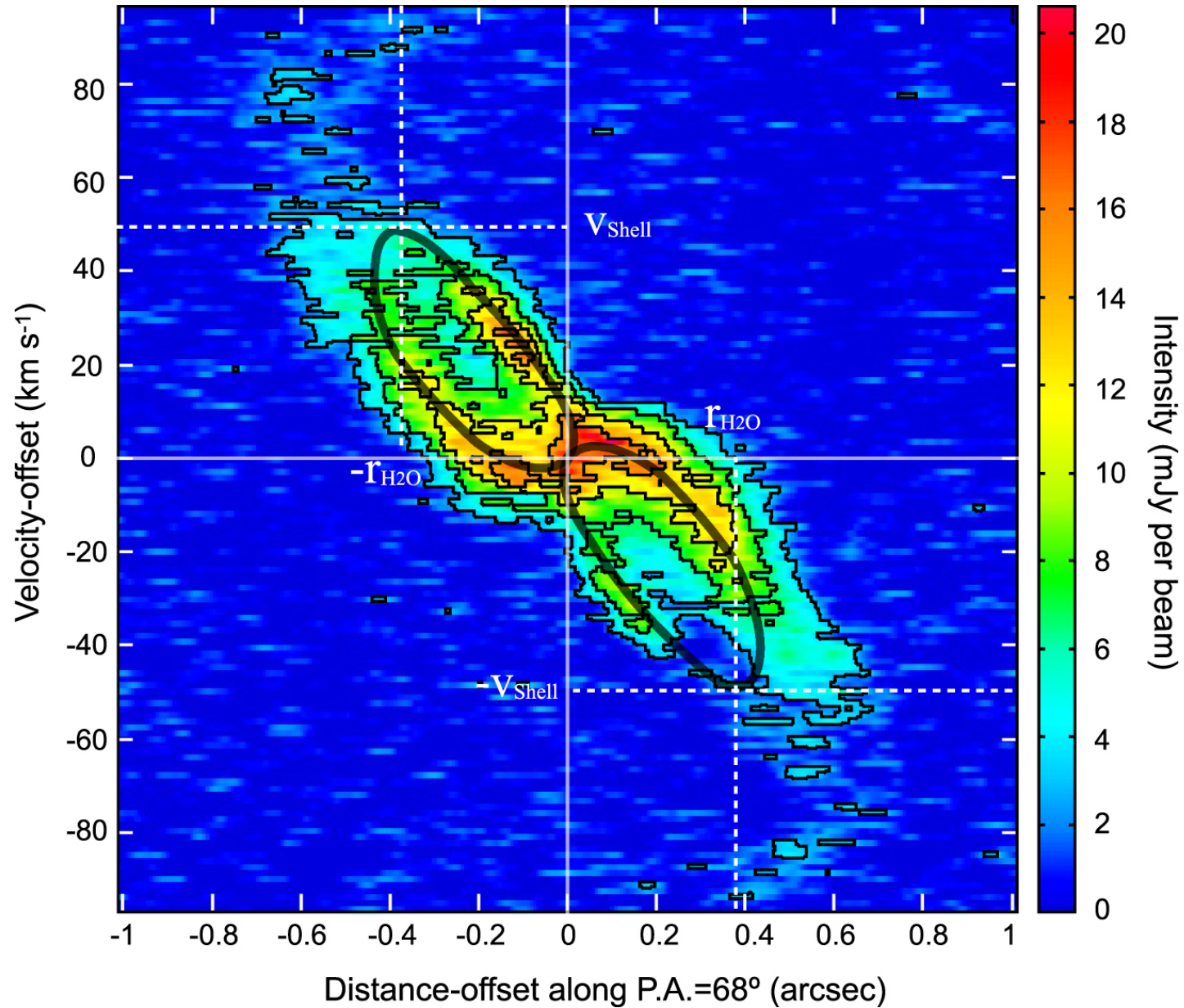
Figure 6. from Shaping the Envelope of the Asymptotic Giant Branch Star W43A with a Collimated Fast Jet null 2020 APJL 890 L14 doi:10.3847/2041-8213/ab70b8 https://dx.doi.org/10.3847/2041-8213/ab70b8 © 2020. The American Astronomical Society. All rights reserved.
