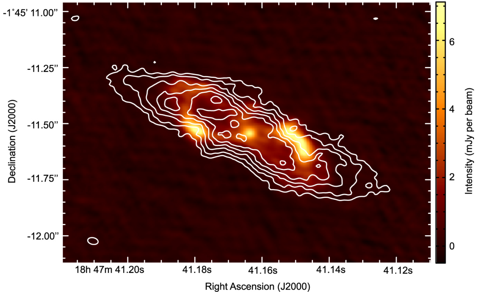
Figure 5. from Shaping the Envelope of the Asymptotic Giant Branch Star W43A with a Collimated Fast Jet null 2020 APJL 890 L14 doi:10.3847/2041-8213/ab70b8 https://dx.doi.org/10.3847/2041-8213/ab70b8 © 2020. The American Astronomical Society. All rights reserved.
