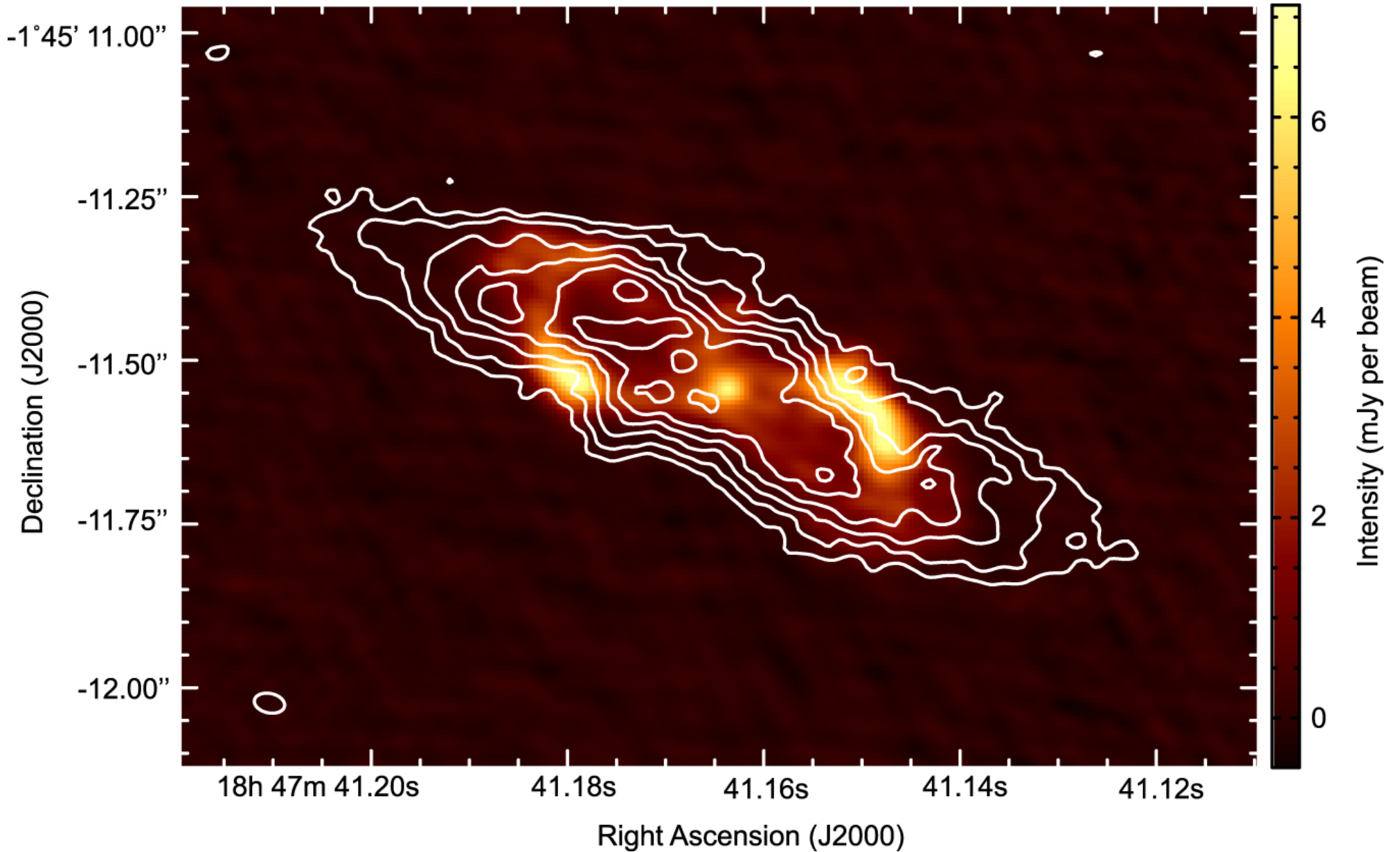
Figure 5. from Shaping the Envelope of the Asymptotic Giant Branch Star W43A with a Collimated Fast Jet null 2020 APJL 890 L14 doi:10.3847/2041-8213/ab70b8 http://dx.doi.org/10.3847/2041-8213/ab70b8 © 2020. The American Astronomical Society. All rights reserved.
