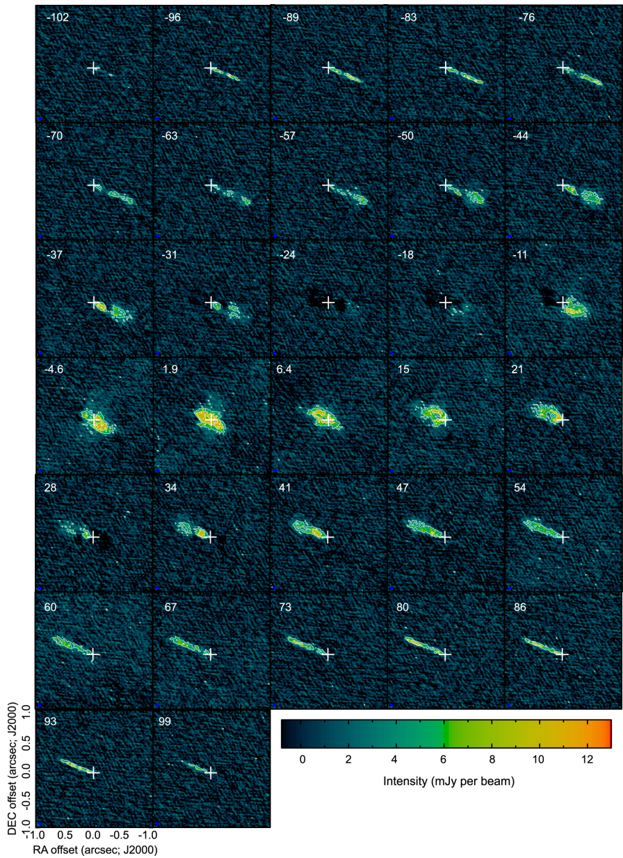
Figure 4. from Shaping the Envelope of the Asymptotic Giant Branch Star W43A with a Collimated Fast Jet null 2020 APJL 890 L14 doi:10.3847/2041-8213/ab70b8 https://dx.doi.org/10.3847/2041-8213/ab70b8 © 2020. The American Astronomical Society. All rights reserved.
