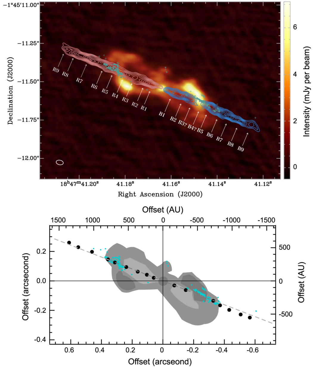
Figure 3. from Shaping the Envelope of the Asymptotic Giant Branch Star W43A with a Collimated Fast Jet null 2020 APJL 890 L14 doi:10.3847/2041-8213/ab70b8 http://dx.doi.org/10.3847/2041-8213/ab70b8 © 2020. The American Astronomical Society. All rights reserved.
