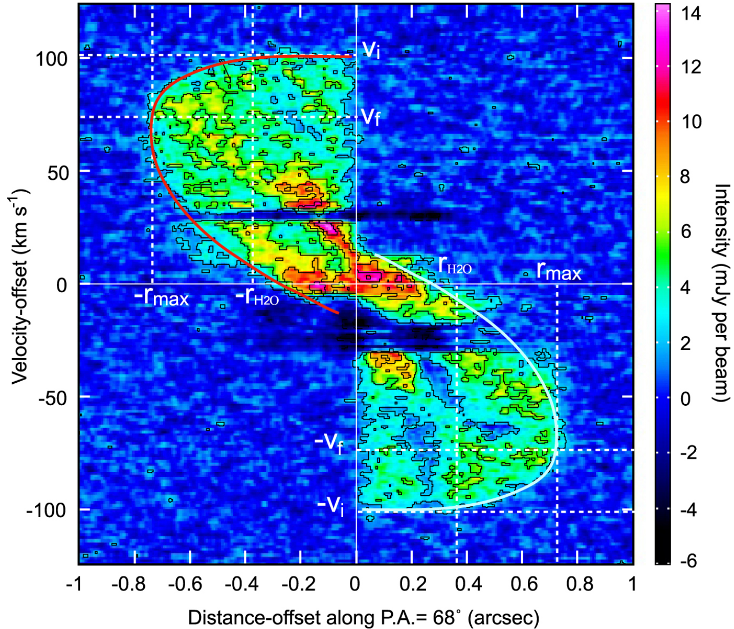
Figure 2. from Shaping the Envelope of the Asymptotic Giant Branch Star W43A with a Collimated Fast Jet null 2020 APJL 890 L14 doi:10.3847/2041-8213/ab70b8 https://dx.doi.org/10.3847/2041-8213/ab70b8 © 2020. The American Astronomical Society. All rights reserved.
