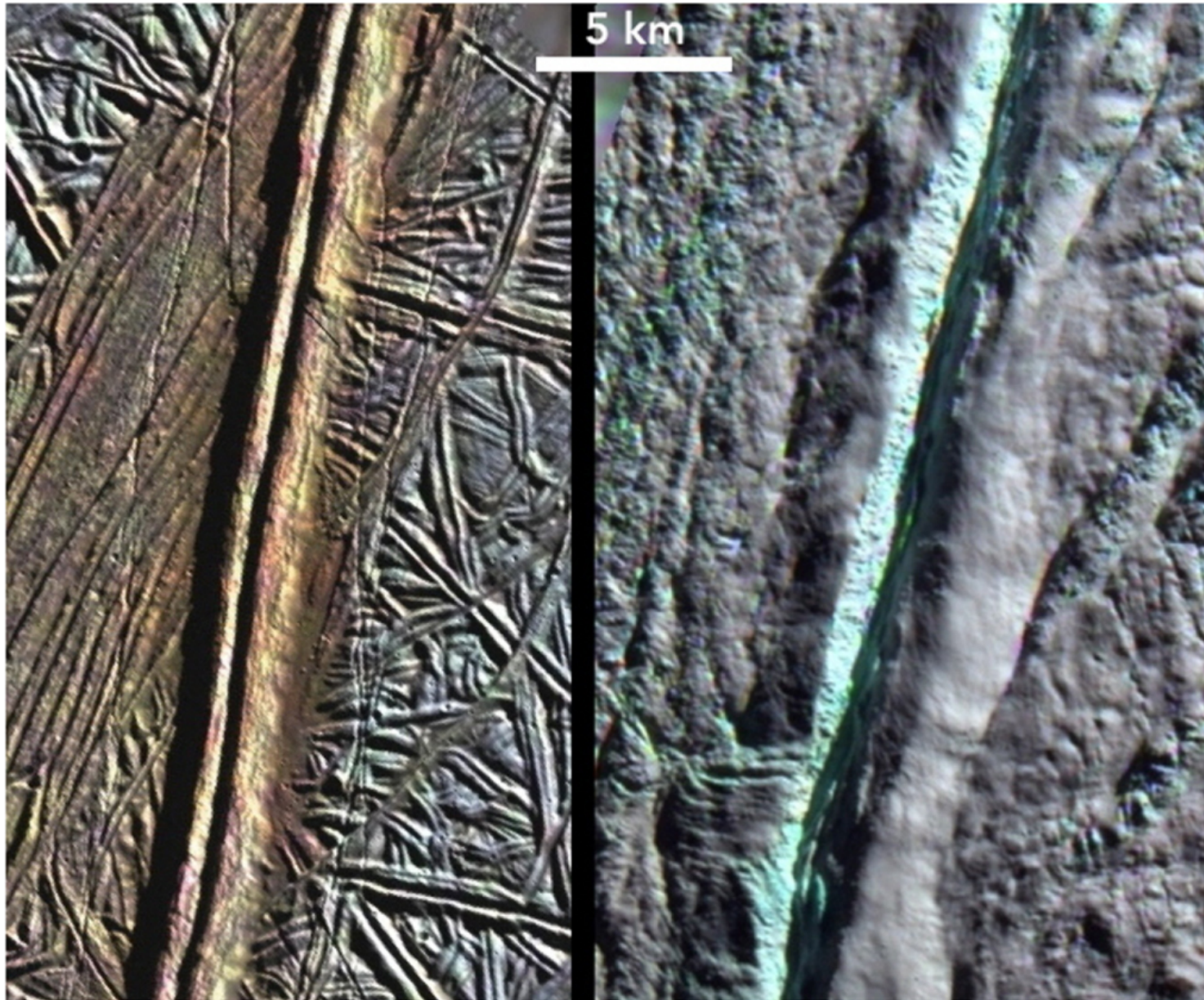
Figure 5. from The Search for Europa's Plumes: No Surface Patterns or Changes 1979–2007? null 2020 APJL 892 L12 doi:10.3847/2041-8213/ab6f78 http://dx.doi.org/10.3847/2041-8213/ab6f78 © 2020. The American Astronomical Society. All rights reserved.
