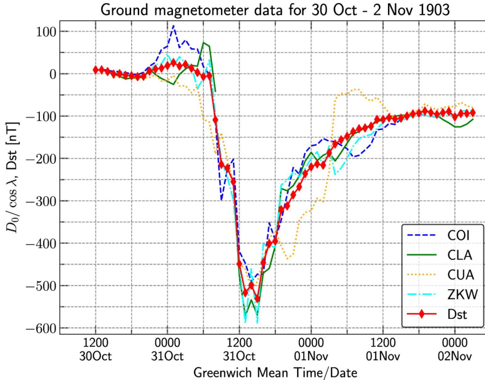
Figure 4. from The Extreme Space Weather Event in 1903 October/November: An Outburst from the Quiet Sun null 2020 APJL 897 L10 doi:10.3847/2041-8213/ab6a18 https://dx.doi.org/10.3847/2041-8213/ab6a18 © 2020. The American Astronomical Society. All rights reserved.
