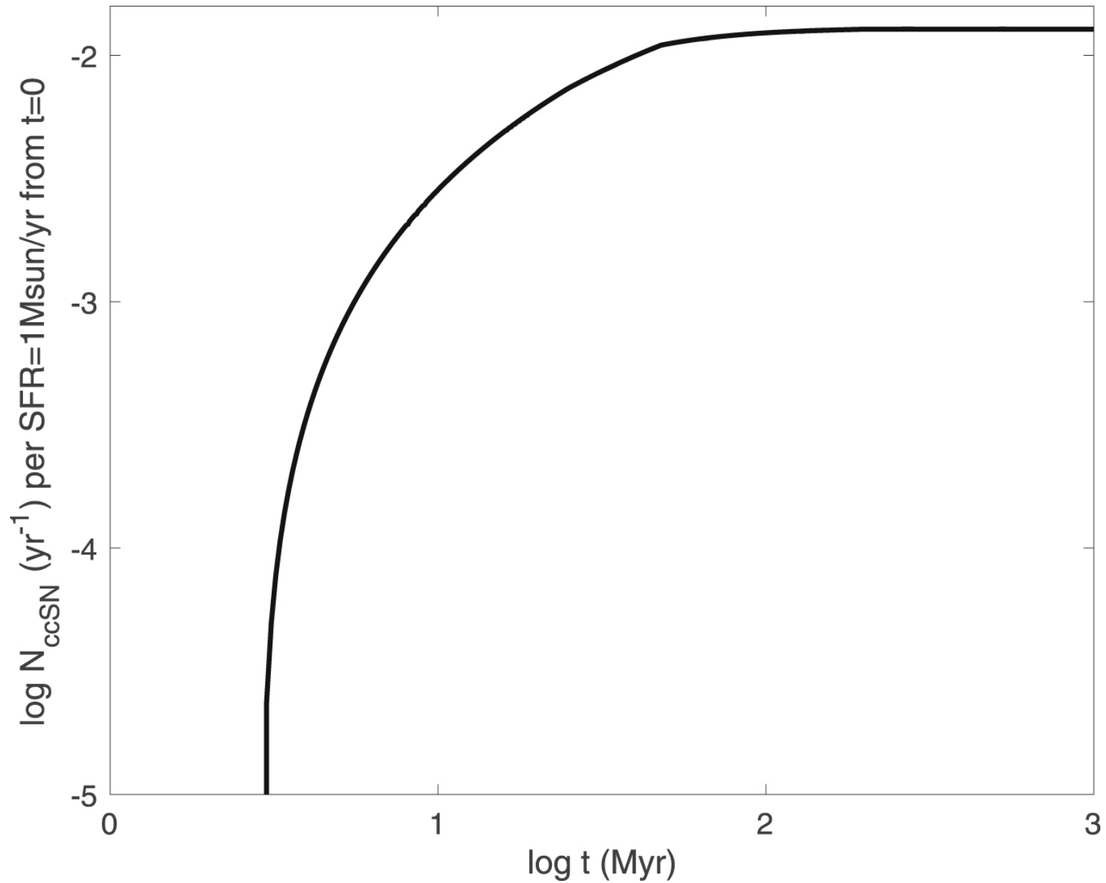
Figure 1. from Physics of Prodigious Lyman Continuum Leakers null 2020 APJL 889 L22 doi:10.3847/2041-8213/ab6560 http://dx.doi.org/10.3847/2041-8213/ab6560 © 2020. The American Astronomical Society. All rights reserved.
