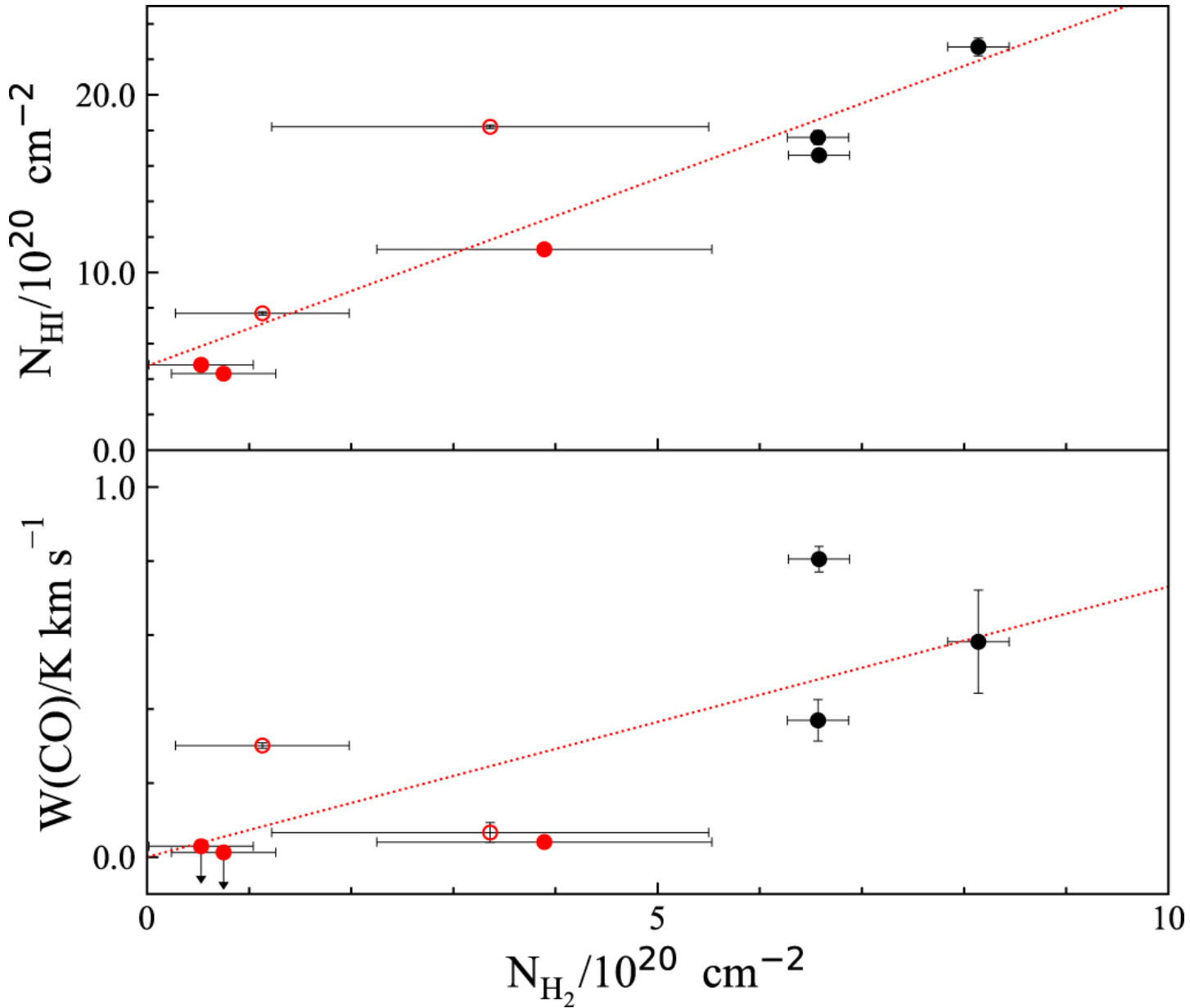
Figure 4. from Revealing the CO X-factor in Dark Molecular Gas through Sensitive ALMA Absorption Observations null 2020 APJL 889 L4 doi:10.3847/2041-8213/ab6337 http://dx.doi.org/10.3847/2041-8213/ab6337 © 2020. The American Astronomical Society. All rights reserved.
