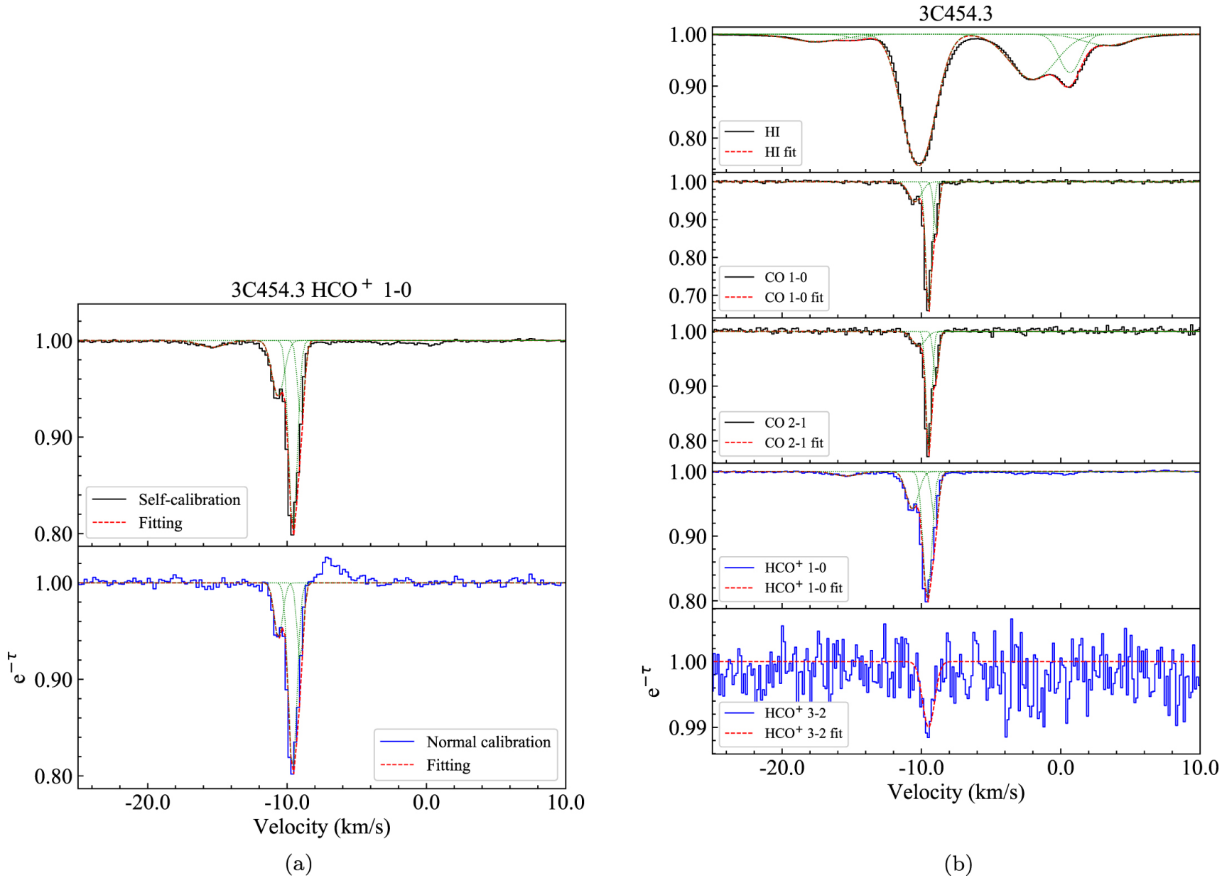
Figure 1. from Revealing the CO X-factor in Dark Molecular Gas through Sensitive ALMA Absorption Observations null 2020 APJL 889 L4 doi:10.3847/2041-8213/ab6337 http://dx.doi.org/10.3847/2041-8213/ab6337 © 2020. The American Astronomical Society. All rights reserved.
