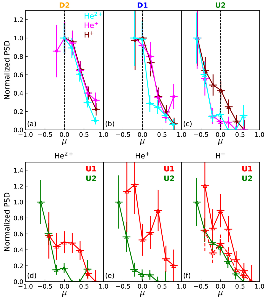
Figure 5. from The Pitch-angle Distributions of Suprathermal Ions near an Interplanetary Shock null 2020 APJL 888 L22 doi:10.3847/2041-8213/ab629d http://dx.doi.org/10.3847/2041-8213/ab629d © 2020. The American Astronomical Society. All rights reserved.
