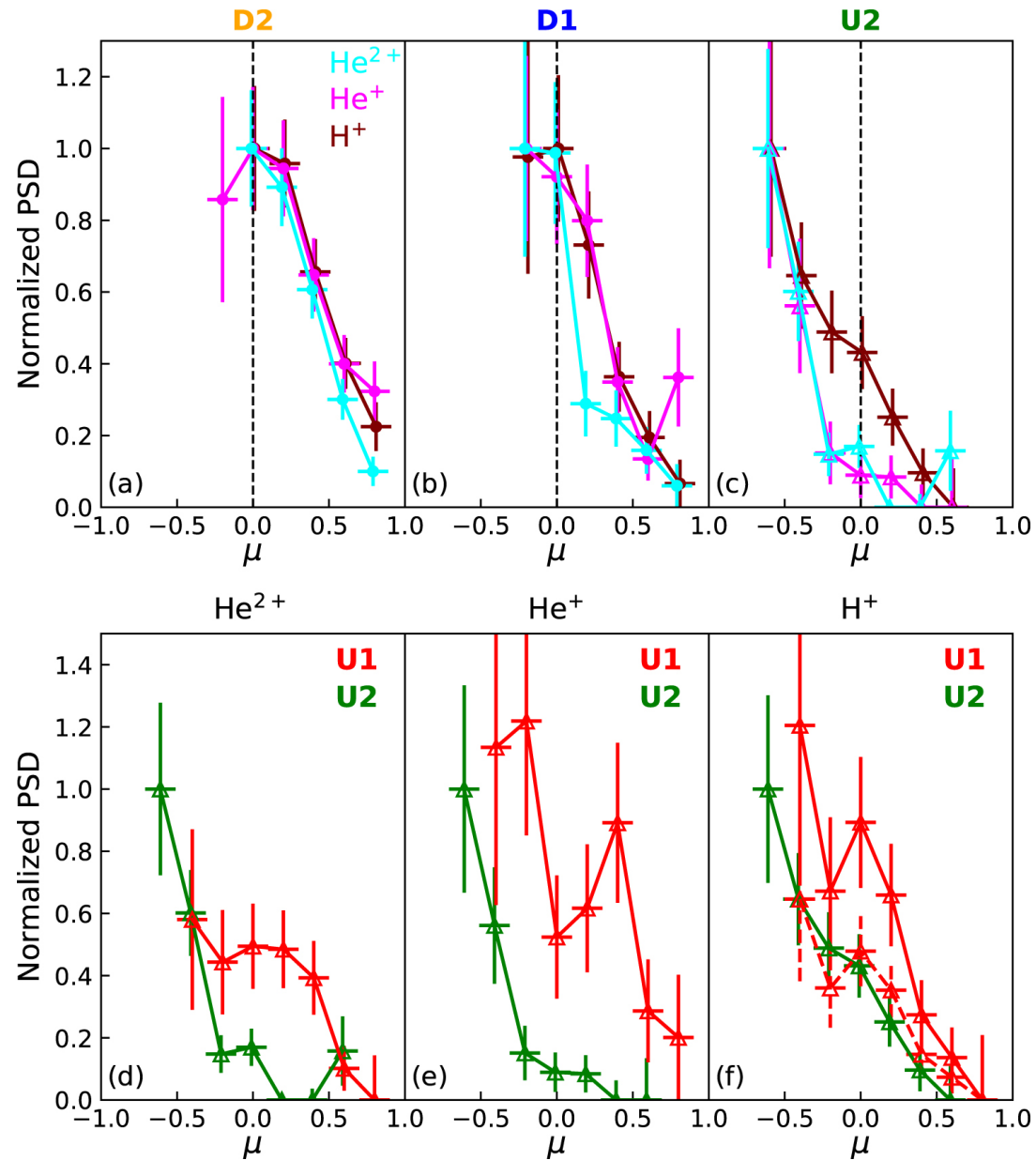
Figure 5. from The Pitch-angle Distributions of Suprathermal Ions near an Interplanetary Shock null 2020 APJL 888 L22 doi:10.3847/2041-8213/ab629d https://dx.doi.org/10.3847/2041-8213/ab629d © 2020. The American Astronomical Society. All rights reserved.
