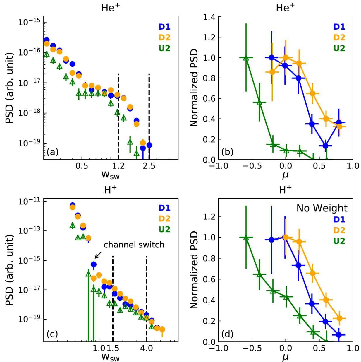
Figure 4. from The Pitch-angle Distributions of Suprathermal Ions near an Interplanetary Shock null 2020 APJL 888 L22 doi:10.3847/2041-8213/ab629d https://dx.doi.org/10.3847/2041-8213/ab629d © 2020. The American Astronomical Society. All rights reserved.
