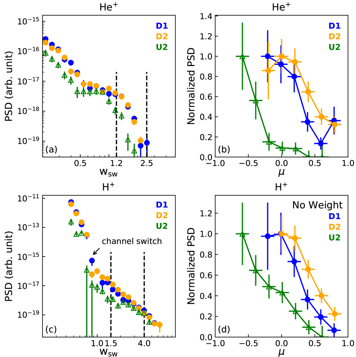
Figure 4. from The Pitch-angle Distributions of Suprathermal Ions near an Interplanetary Shock null 2020 APJL 888 L22 doi:10.3847/2041-8213/ab629d http://dx.doi.org/10.3847/2041-8213/ab629d © 2020. The American Astronomical Society. All rights reserved.
