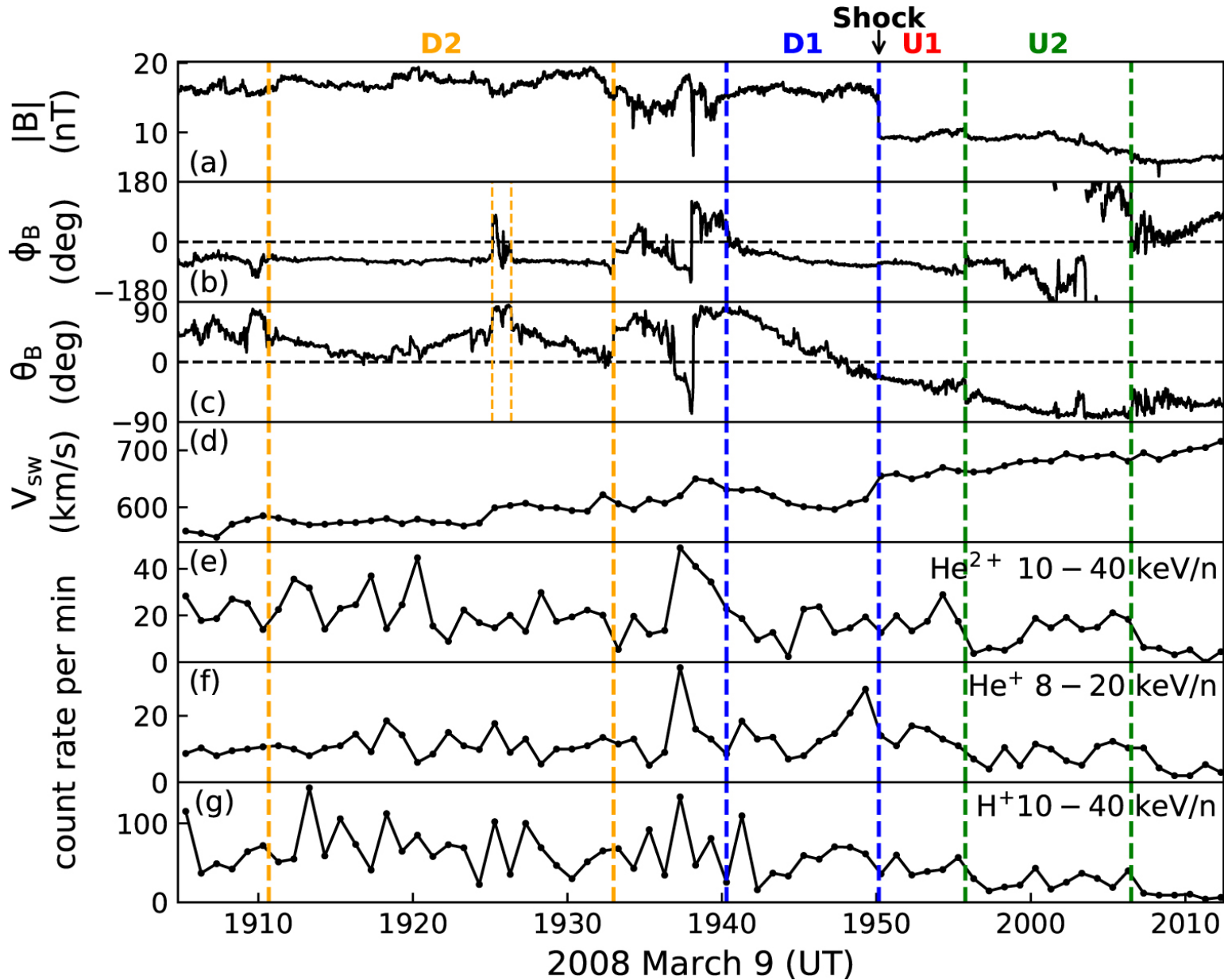
Figure 2. from The Pitch-angle Distributions of Suprathermal Ions near an Interplanetary Shock null 2020 APJL 888 L22 doi:10.3847/2041-8213/ab629d http://dx.doi.org/10.3847/2041-8213/ab629d © 2020. The American Astronomical Society. All rights reserved.
