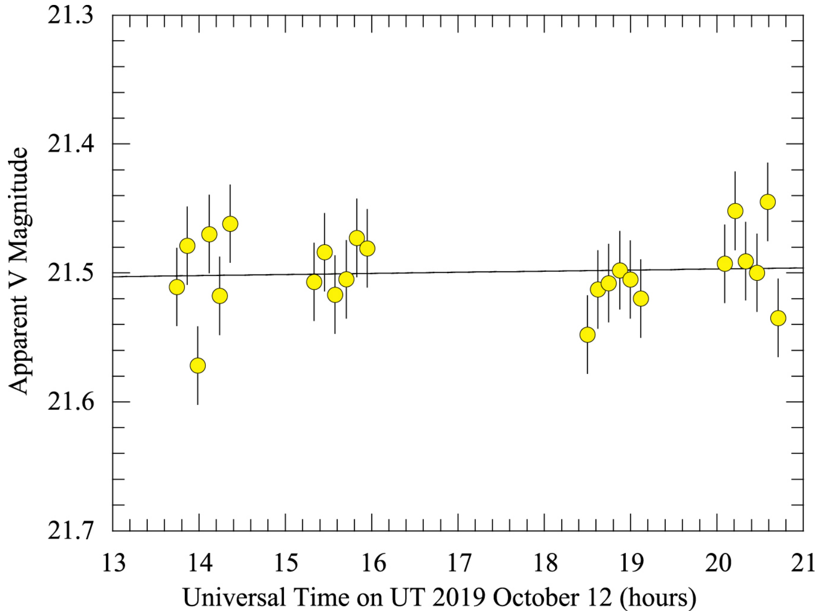
Figure 3. from The Nucleus of Interstellar Comet 2I/Borisov null 2020 APJL 888 L23 doi:10.3847/2041-8213/ab621b http://dx.doi.org/10.3847/2041-8213/ab621b © 2020. The American Astronomical Society. All rights reserved.
