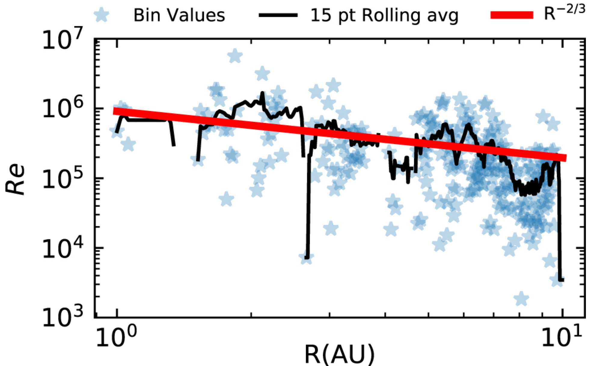
Figure 1. from Reynolds Number and Intermittency in the Expanding Solar Wind: Predictions Based on Voyager Observations null 2019 APJL 884 L57 doi:10.3847/2041-8213/ab4a82 https://dx.doi.org/10.3847/2041-8213/ab4a82 © 2019. The American Astronomical Society. All rights reserved.
