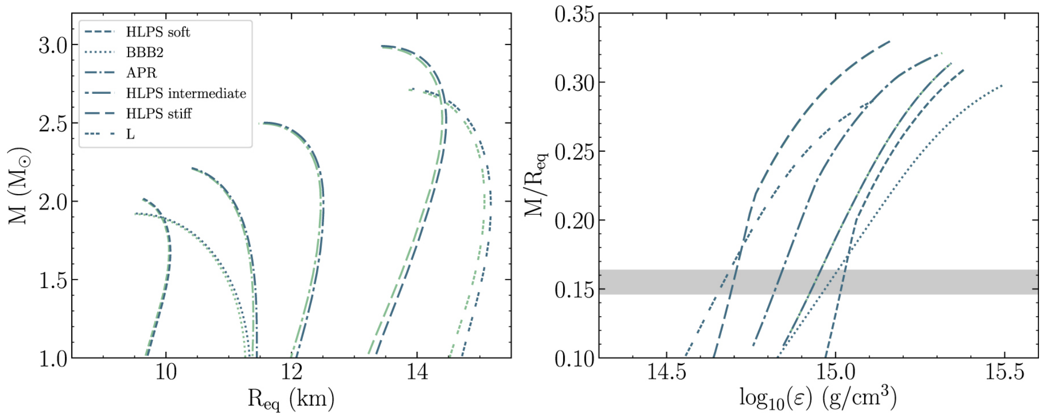
Figure 5. from A NICER View of PSR J0030+0451: Implications for the Dense Matter Equation of State null 2019 APJL 887 L22 doi:10.3847/2041-8213/ab451a https://dx.doi.org/10.3847/2041-8213/ab451a © 2019. The American Astronomical Society. All rights reserved.
