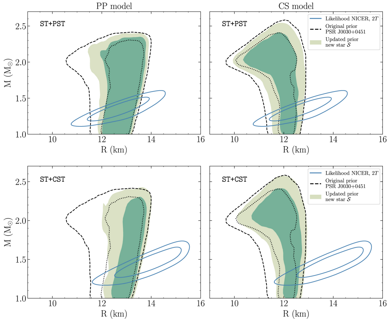
Figure 4. from A NICER View of PSR J0030+0451: Implications for the Dense Matter Equation of State null 2019 APJL 887 L22 doi:10.3847/2041-8213/ab451a https://dx.doi.org/10.3847/2041-8213/ab451a © 2019. The American Astronomical Society. All rights reserved.
