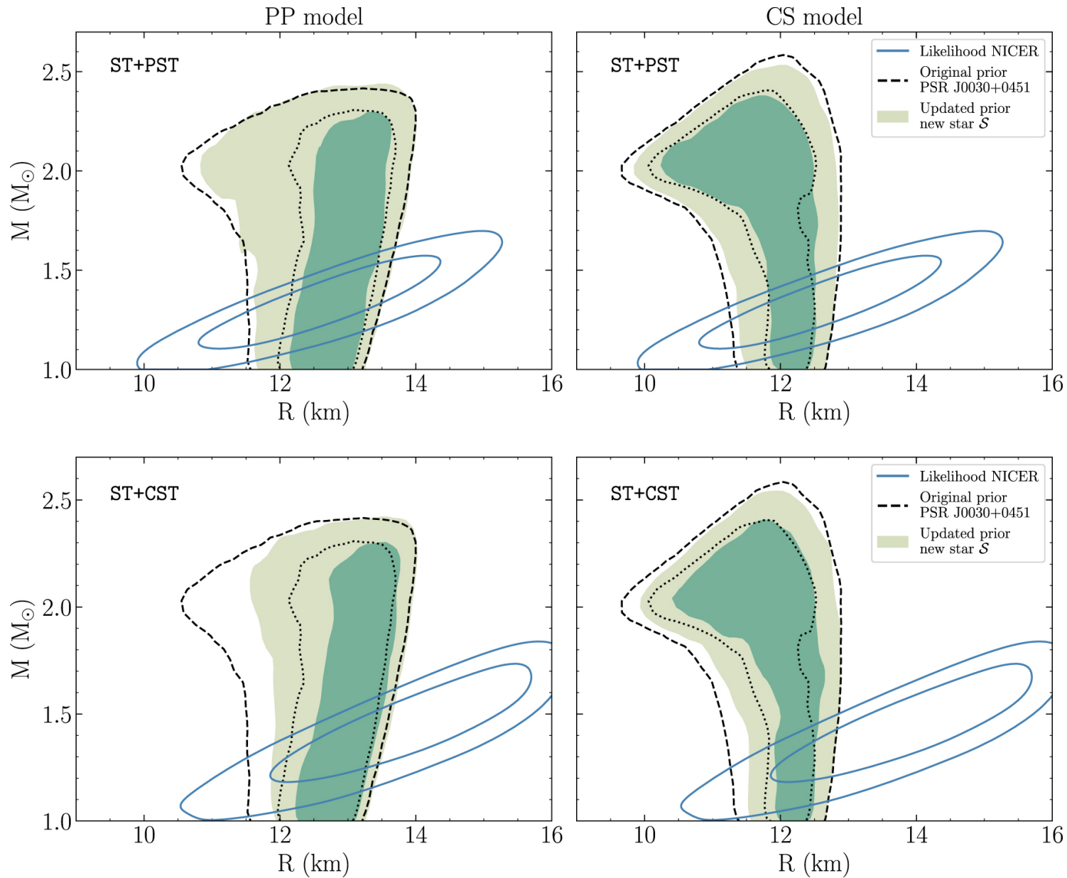
Figure 3. from A NICER View of PSR J0030+0451: Implications for the Dense Matter Equation of State null 2019 APJL 887 L22 doi:10.3847/2041-8213/ab451a https://dx.doi.org/10.3847/2041-8213/ab451a © 2019. The American Astronomical Society. All rights reserved.
