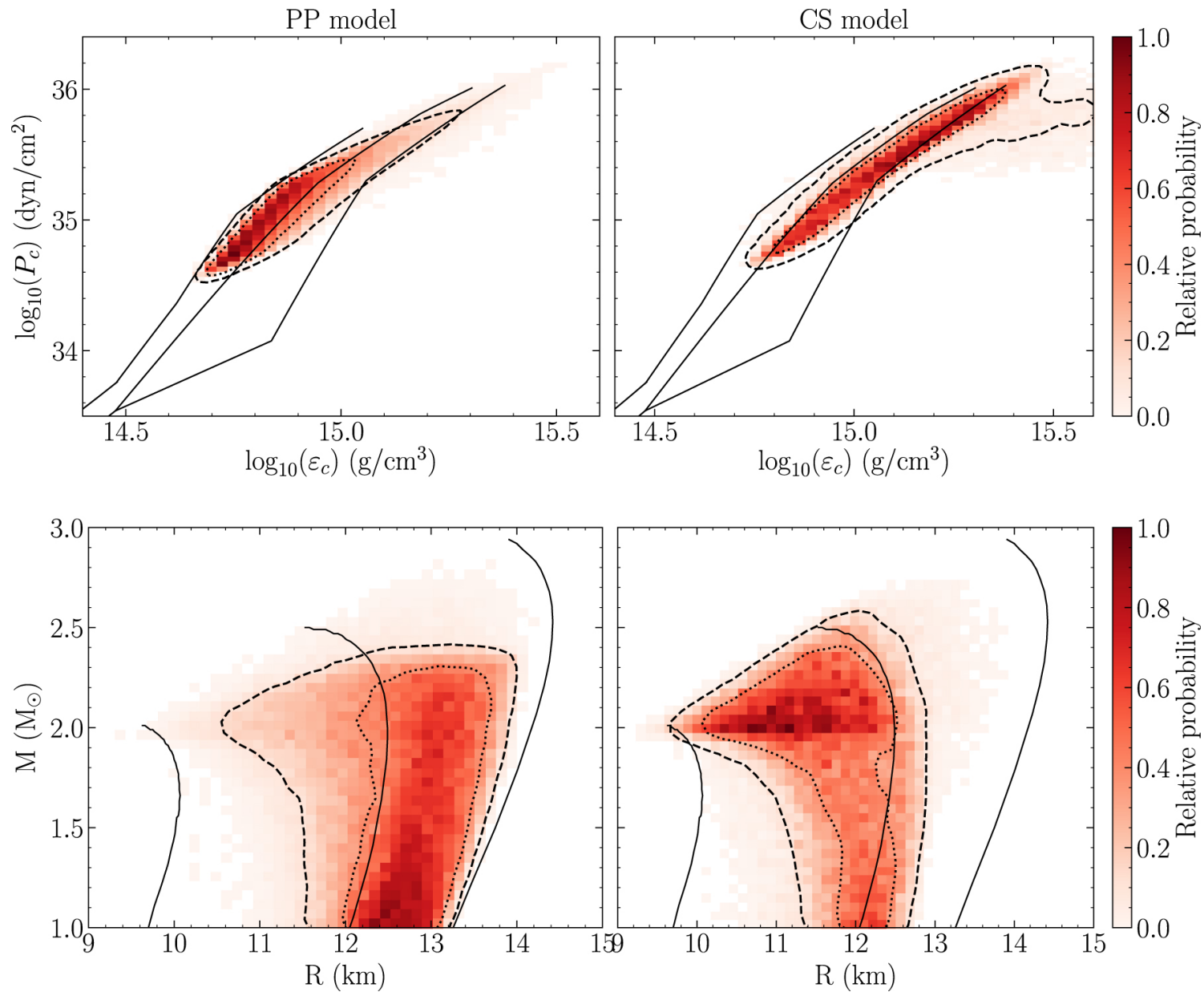
Figure 1. from A NICER View of PSR J0030+0451: Implications for the Dense Matter Equation of State null 2019 APJL 887 L22 doi:10.3847/2041-8213/ab451a https://dx.doi.org/10.3847/2041-8213/ab451a © 2019. The American Astronomical Society. All rights reserved.
