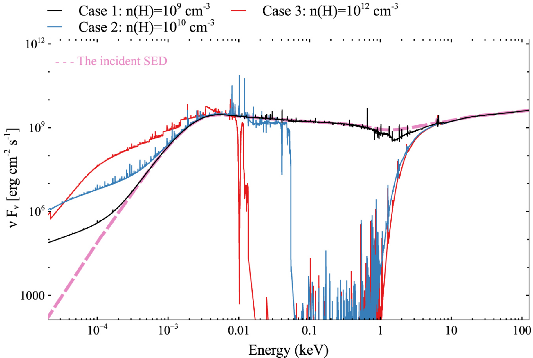
Figure 3. from A Wind-based Unification Model for NGC 5548: Spectral Holidays, Nondisk Emission, and Implications for Changing-look Quasars null 2019 APJL 882 L30 doi:10.3847/2041-8213/ab3d41 https://dx.doi.org/10.3847/2041-8213/ab3d41 © 2019. The American Astronomical Society. All rights reserved.
