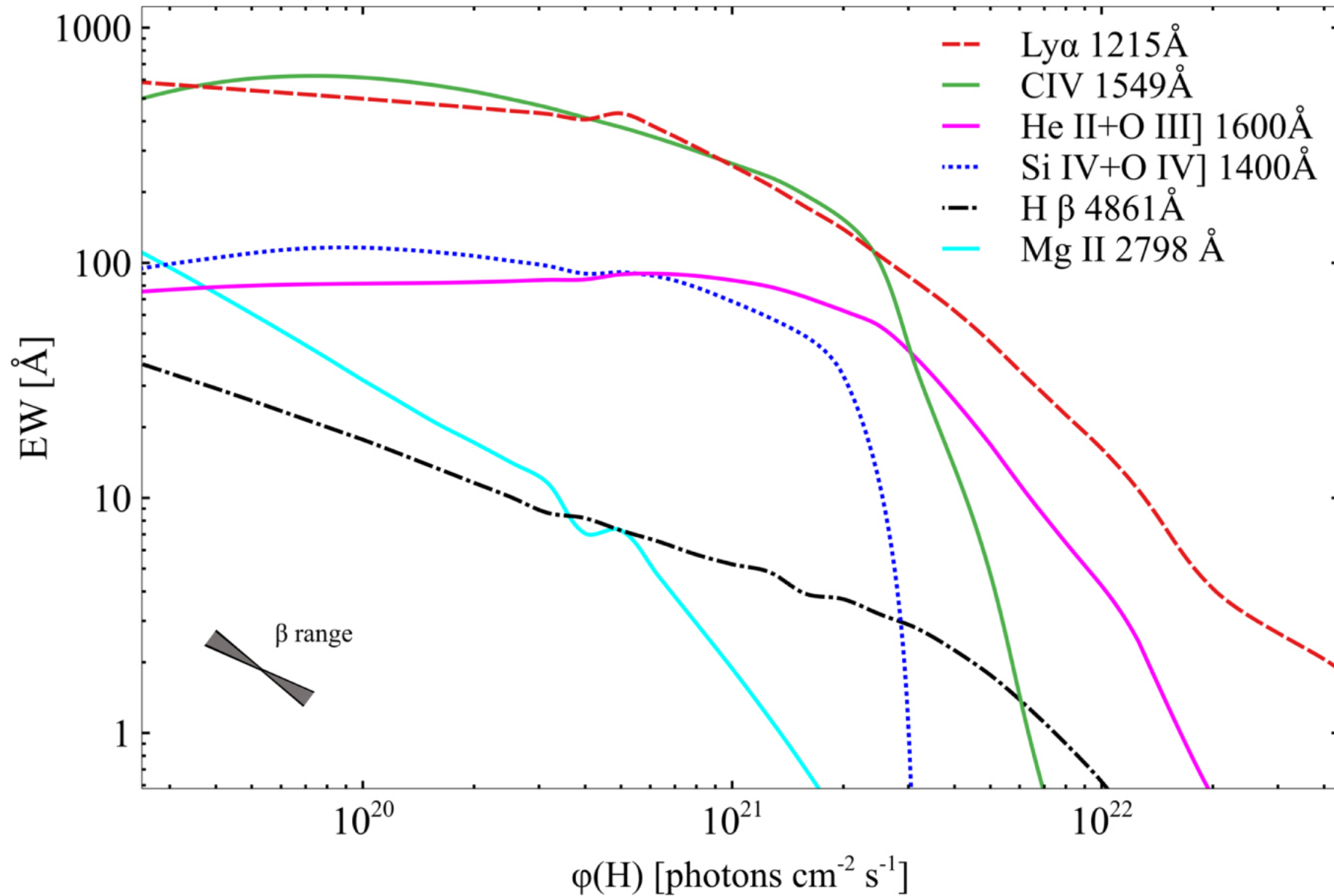
Figure 2. from A Wind-based Unification Model for NGC 5548: Spectral Holidays, Nondisk Emission, and Implications for Changing-look Quasars null 2019 APJL 882 L30 doi:10.3847/2041-8213/ab3d41 https://dx.doi.org/10.3847/2041-8213/ab3d41 © 2019. The American Astronomical Society. All rights reserved.
