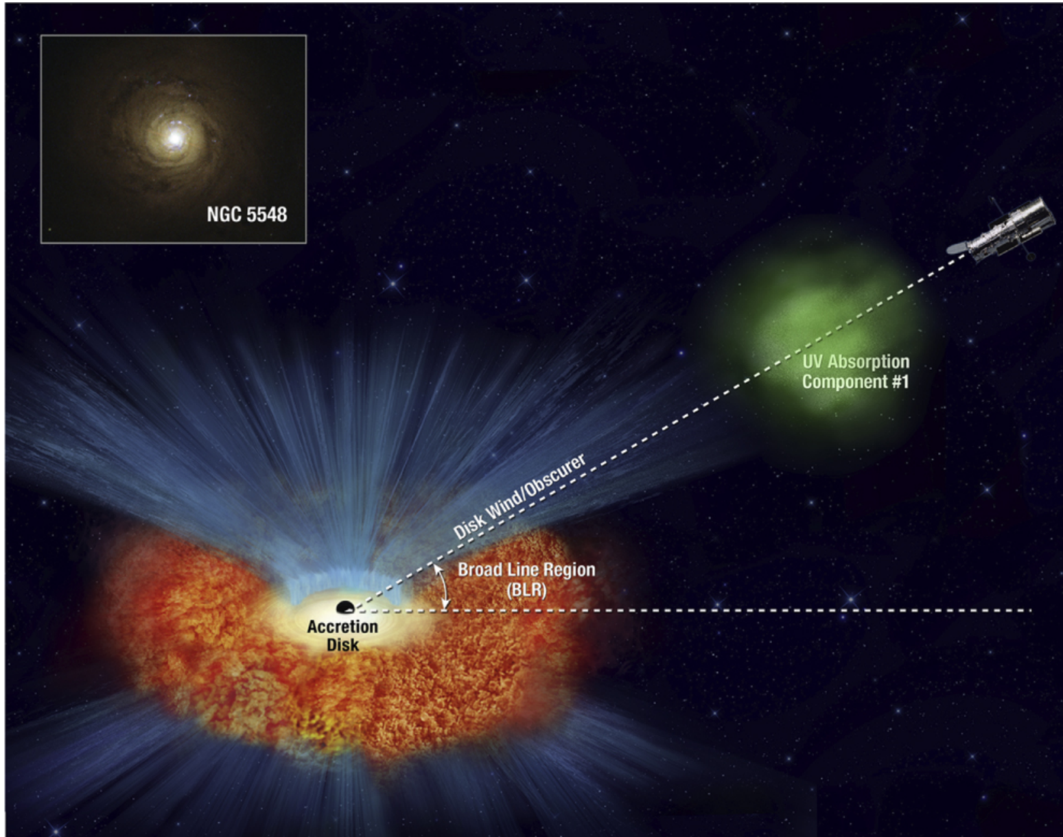
Figure 1. from A Wind-based Unification Model for NGC 5548: Spectral Holidays, Nondisk Emission, and Implications for Changing-look Quasars null 2019 APJL 882 L30 doi:10.3847/2041-8213/ab3d41 https://dx.doi.org/10.3847/2041-8213/ab3d41 © 2019. The American Astronomical Society. All rights reserved.
