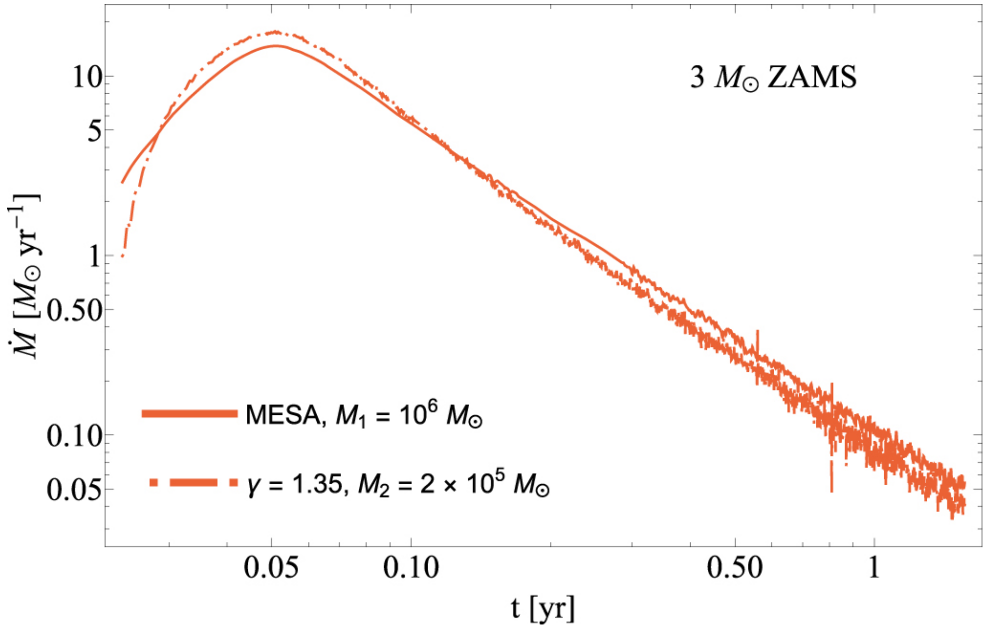
Figure 8. from On the Diversity of Fallback Rates from Tidal Disruption Events with Accurate Stellar Structure null 2019 APJL 882 L26 doi:10.3847/2041-8213/ab380d https://dx.doi.org/10.3847/2041-8213/ab380d © 2019. The American Astronomical Society. All rights reserved.
