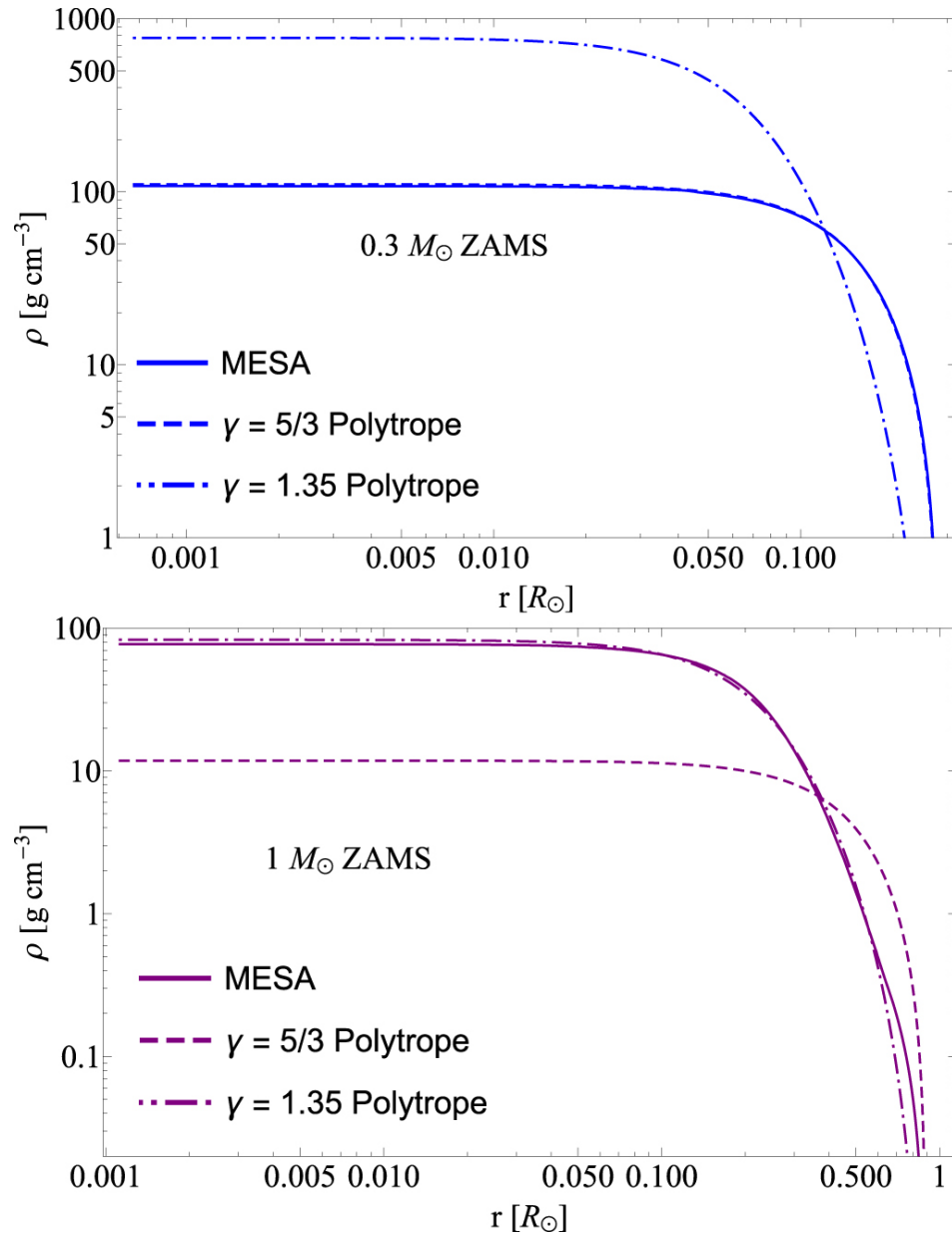
Figure 5. from On the Diversity of Fallback Rates from Tidal Disruption Events with Accurate Stellar Structure null 2019 APJL 882 L26 doi:10.3847/2041-8213/ab380d https://dx.doi.org/10.3847/2041-8213/ab380d
