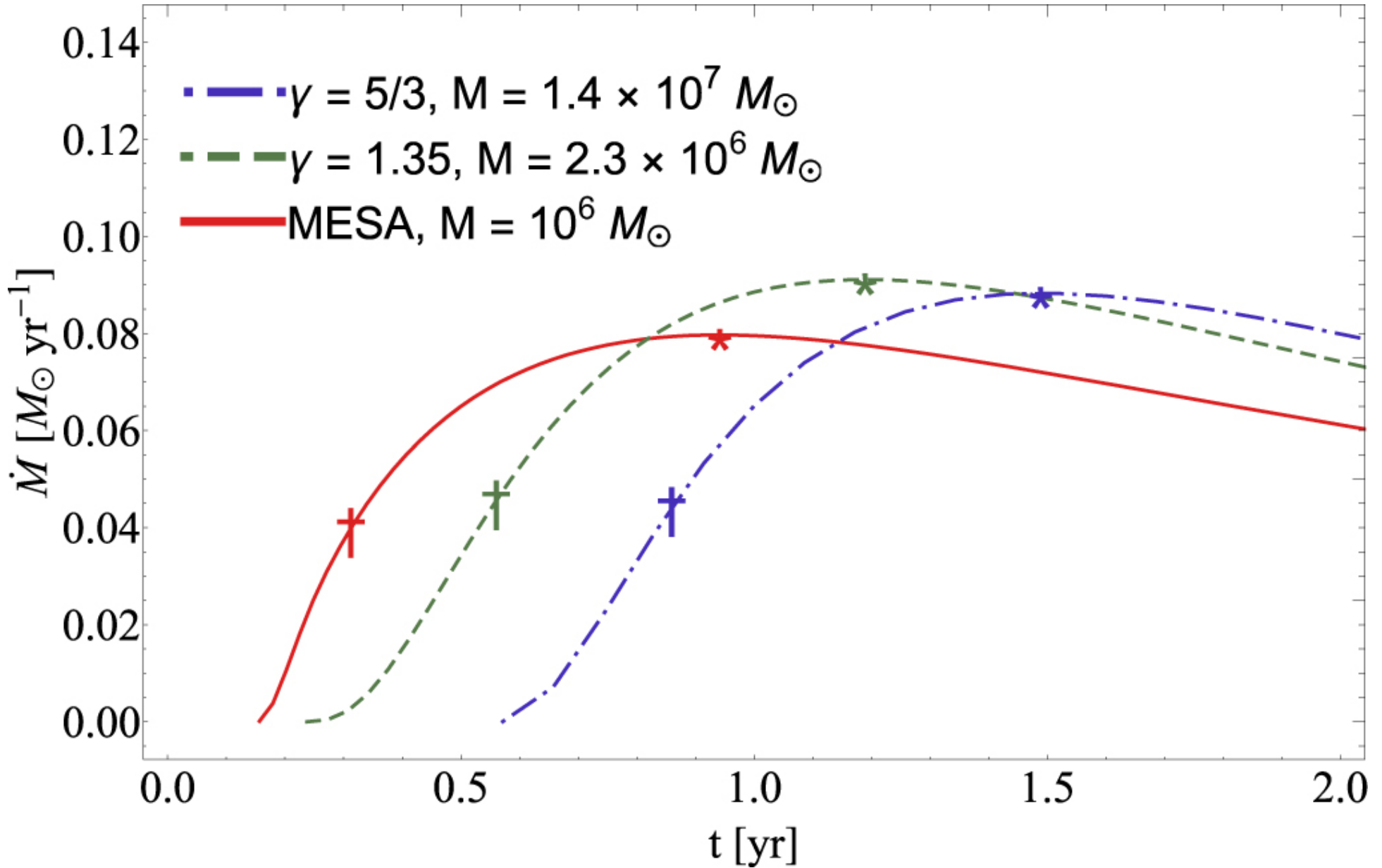
Figure 3. from On the Diversity of Fallback Rates from Tidal Disruption Events with Accurate Stellar Structure null 2019 APJL 882 L26 doi:10.3847/2041-8213/ab380d http://dx.doi.org/10.3847/2041-8213/ab380d © 2019. The American Astronomical Society. All rights reserved.
