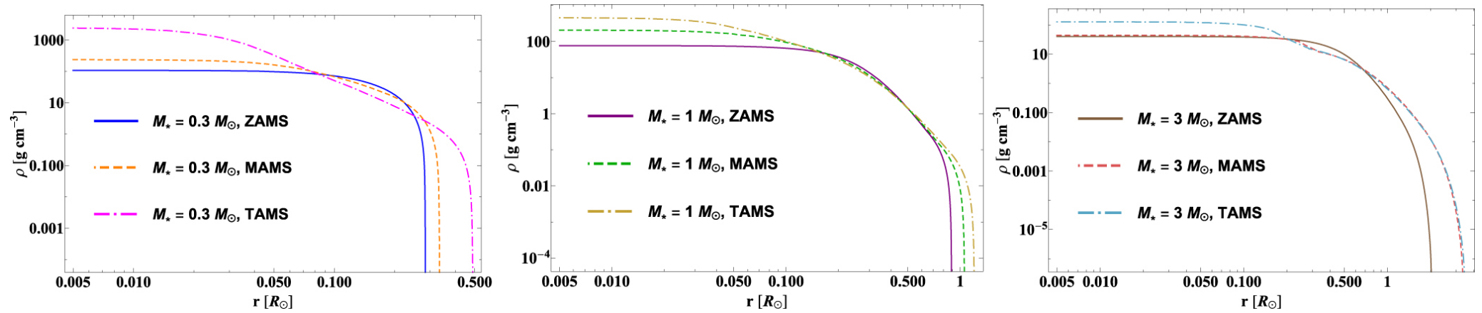
Figure 1. from On the Diversity of Fallback Rates from Tidal Disruption Events with Accurate Stellar Structure null 2019 APJL 882 L26 doi:10.3847/2041-8213/ab380d https://dx.doi.org/10.3847/2041-8213/ab380d © 2019. The American Astronomical Society. All rights reserved.
