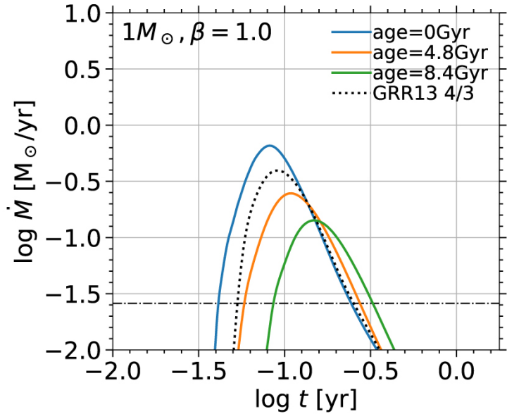
Figure 3. from The Tidal Disruption of Sun-like Stars by Massive Black Holes null 2019 APJL 882 L25 doi:10.3847/2041-8213/ab379a http://dx.doi.org/10.3847/2041-8213/ab379a
