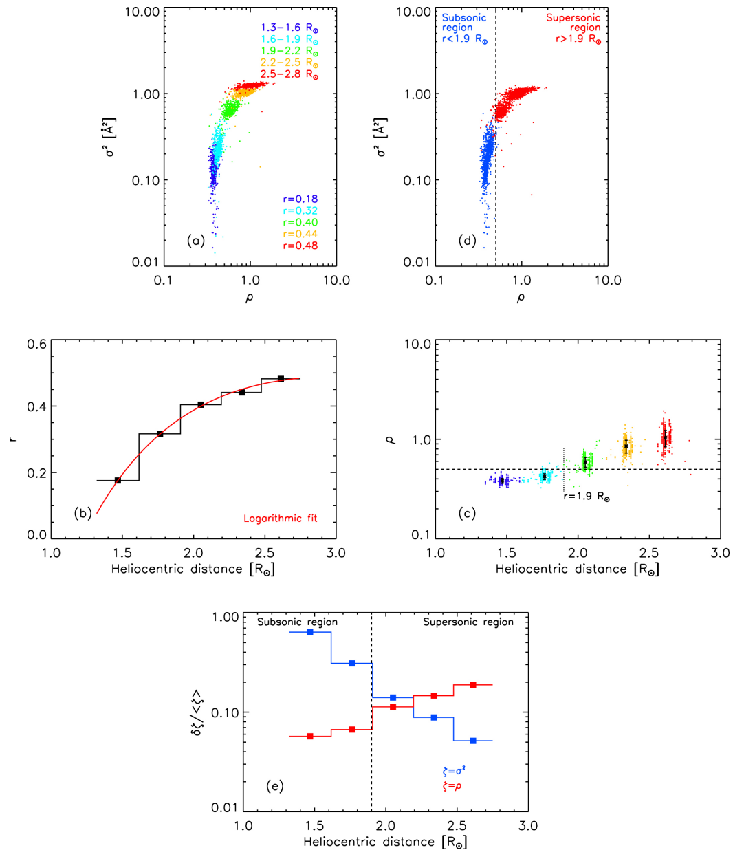
Figure 2. from On the Fast Solar Wind Heating and Acceleration Processes: A Statistical Study Based on the UVCS Survey Data null 2019 APJL 881 L36 doi:10.3847/2041-8213/ab3731 https://dx.doi.org/10.3847/2041-8213/ab3731 © 2019. The American Astronomical Society. All rights reserved.
