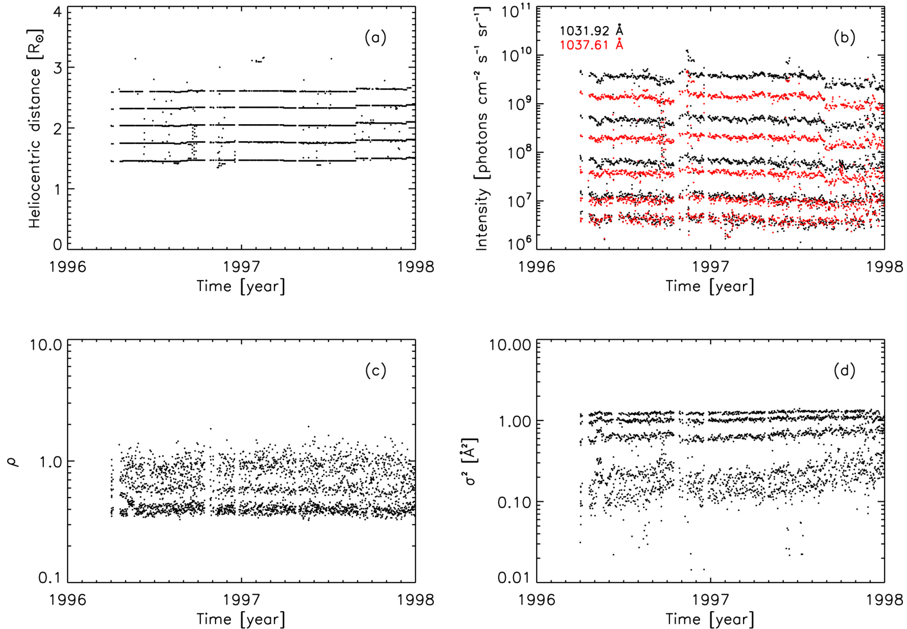
Figure 1. from On the Fast Solar Wind Heating and Acceleration Processes: A Statistical Study Based on the UVCS Survey Data null 2019 APJL 881 L36 doi:10.3847/2041-8213/ab3731 https://dx.doi.org/10.3847/2041-8213/ab3731 © 2019. The American Astronomical Society. All rights reserved.
