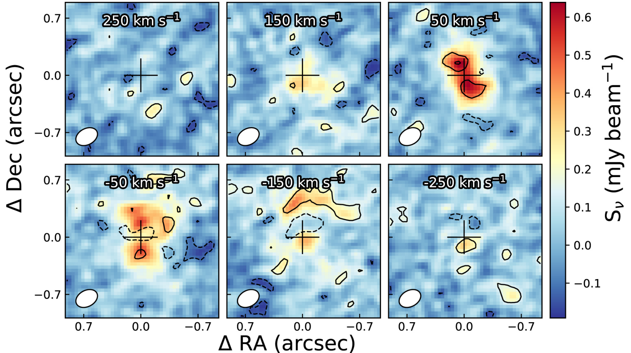
Figure 6. from The z = 7.54 Quasar ULAS J1342+0928 Is Hosted by a Galaxy Merger null 2019 APJL 881 L23 doi:10.3847/2041-8213/ab3659 http://dx.doi.org/10.3847/2041-8213/ab3659 © 2019. The American Astronomical Society. All rights reserved.
