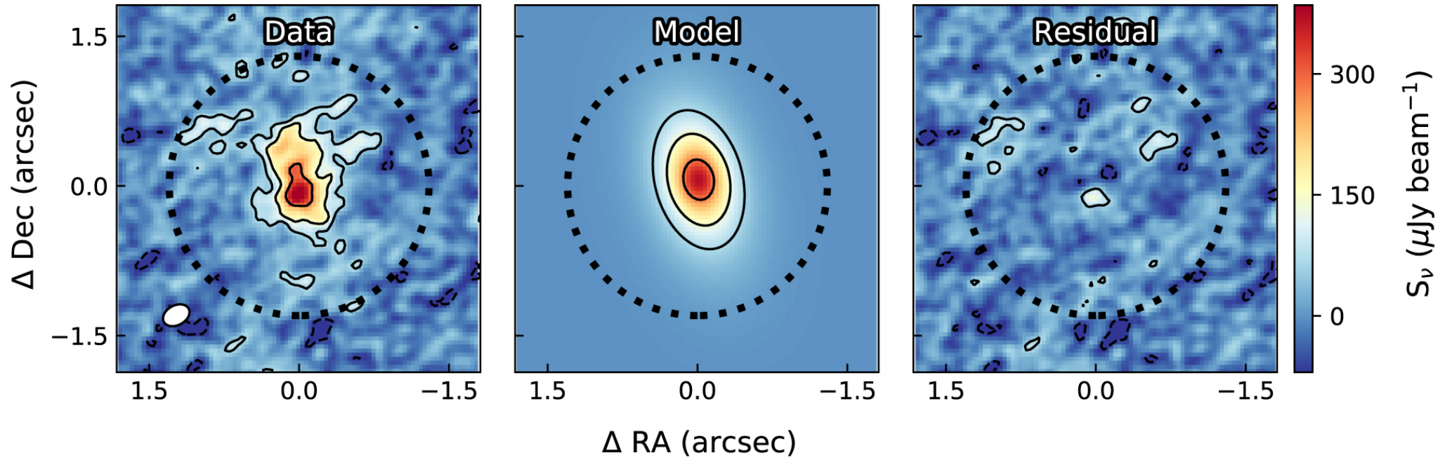
Figure 5. from The z = 7.54 Quasar ULAS J1342+0928 Is Hosted by a Galaxy Merger null 2019 APJL 881 L23 doi:10.3847/2041-8213/ab3659 http://dx.doi.org/10.3847/2041-8213/ab3659 © 2019. The American Astronomical Society. All rights reserved.
