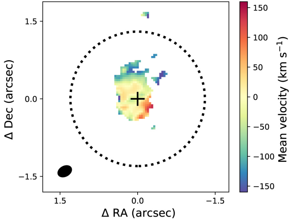
Figure 4. from The z = 7.54 Quasar ULAS J1342+0928 Is Hosted by a Galaxy Merger null 2019 APJL 881 L23 doi:10.3847/2041-8213/ab3659 http://dx.doi.org/10.3847/2041-8213/ab3659 © 2019. The American Astronomical Society. All rights reserved.
